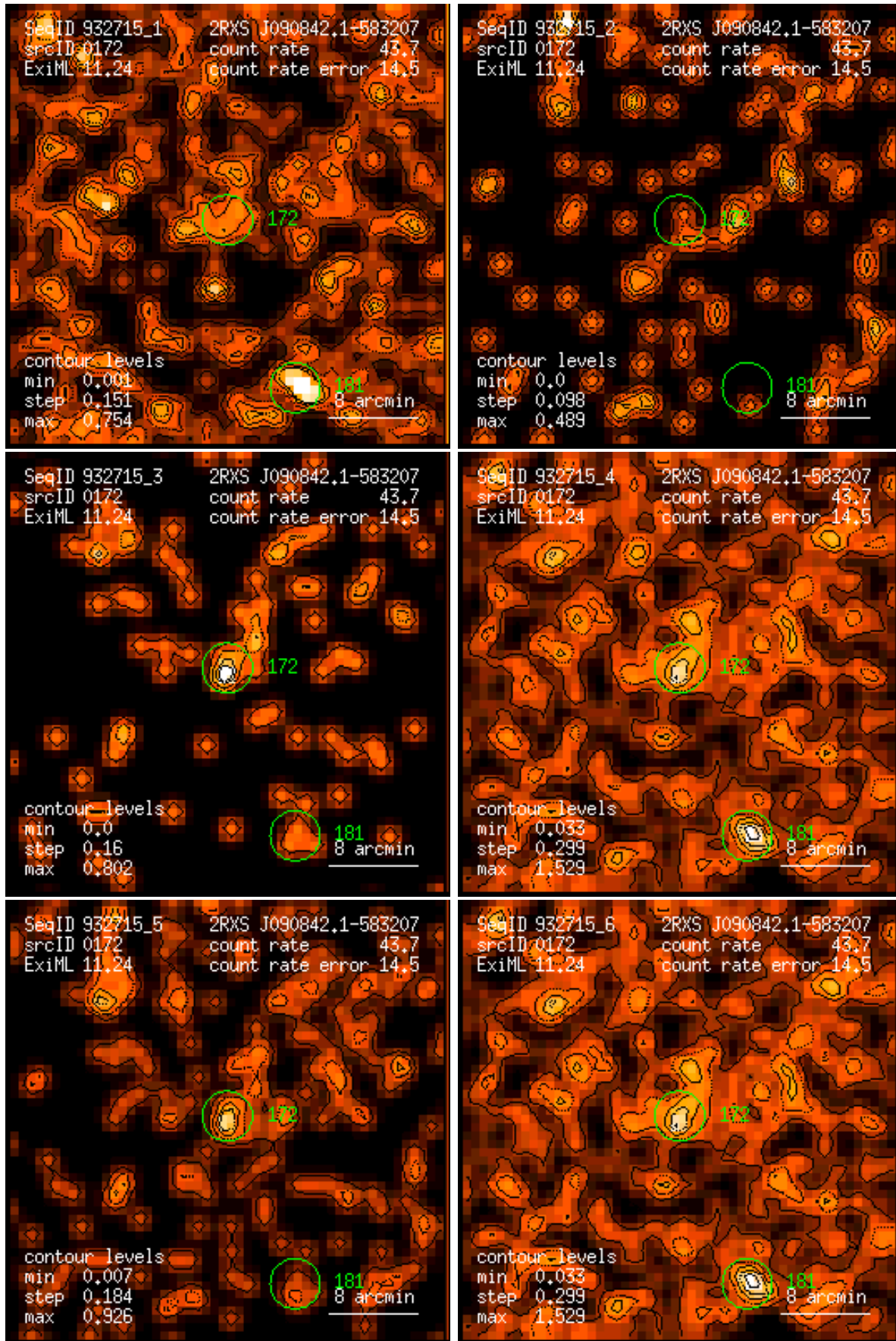
Figure 172: RASS 932715: detection 0172: band rate images, Gaussian filter: (1) PSPC channels 11 – 41, (2) 52 – 90, (3) 91 – 201, (4) 11 – 235, (5) 52 – 201, (6) 11 – 201. Broad band rates in counts/ks. Band rate contour levels in counts/ks/arcmin 2 .
