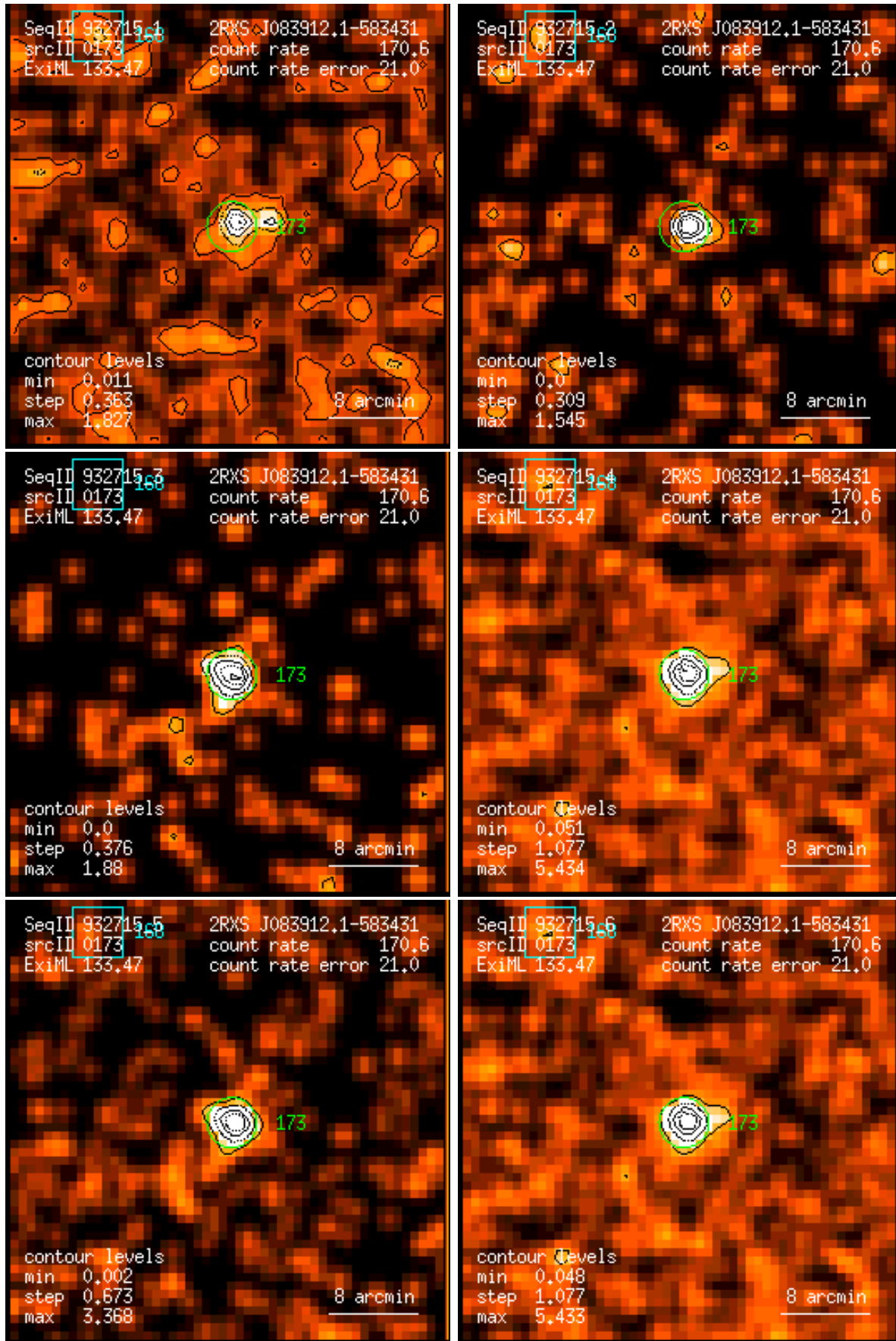
Figure 173: RASS 932715: detection 0173: band rate images, Gaussian filter: (1) PSPC channels 11 – 41, (2) 52 – 90, (3) 91 – 201, (4) 11 – 235, (5) 52 – 201, (6) 11 – 201. Broad band rates in counts/ks. Band rate contour levels in counts/ks/arcmin 2 .
