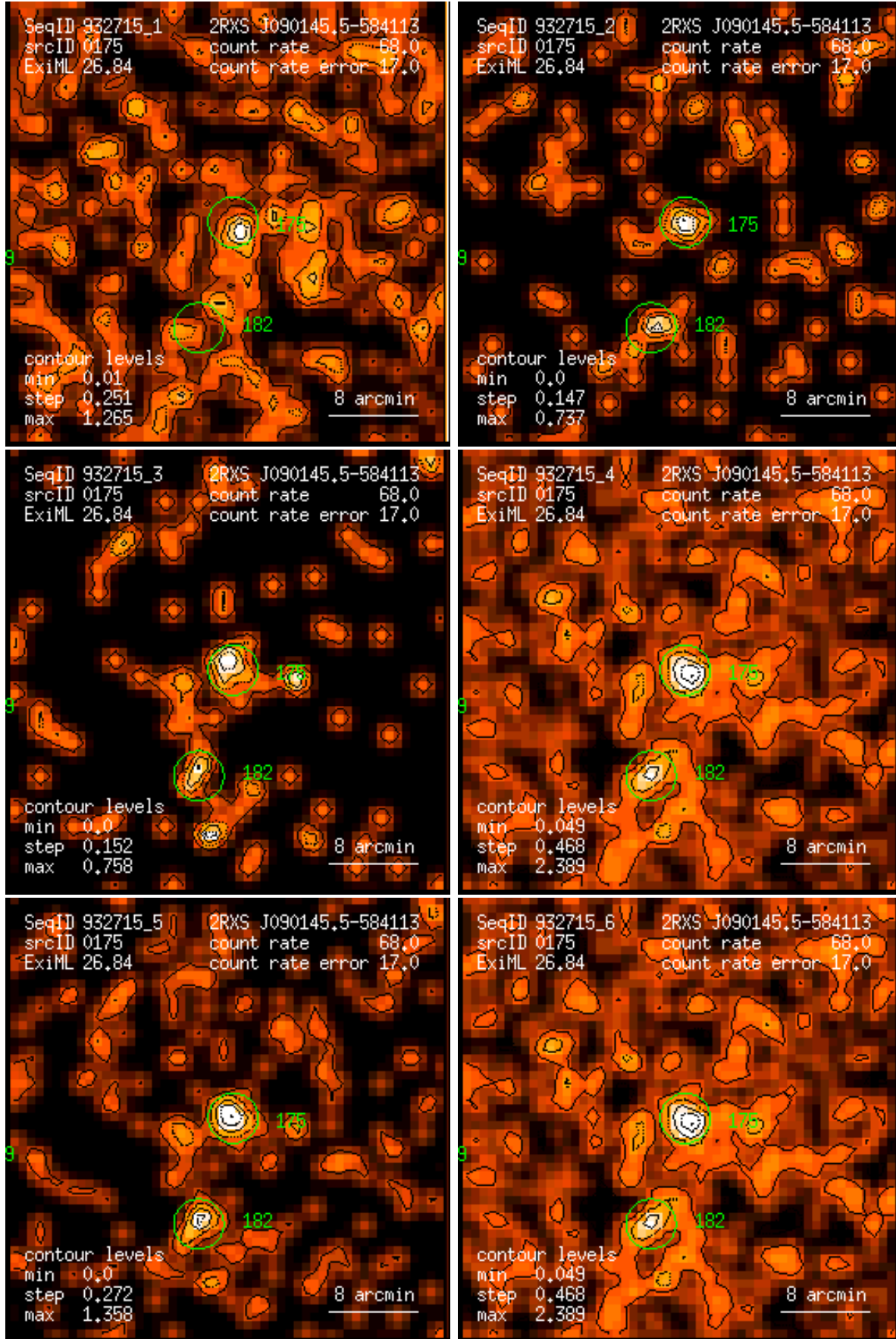
Figure 175: RASS 932715: detection 0175: band rate images, Gaussian filter: (1) PSPC channels 11 – 41, (2) 52 – 90, (3) 91 – 201, (4) 11 – 235, (5) 52 – 201, (6) 11 – 201. Broad band rates in counts/ks. Band rate contour levels in counts/ks/arcmin 2 .
