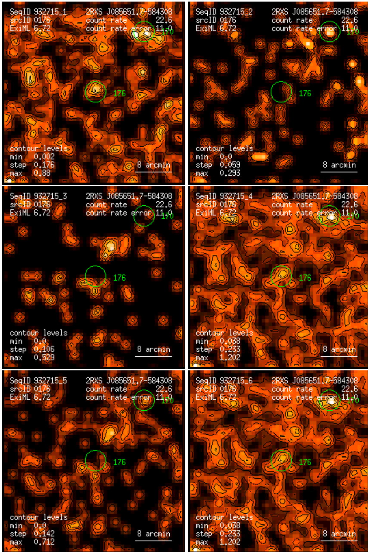
Figure 176: RASS 932715: detection 0176: band rate images, Gaussian filter: (1) PSPC channels 11 – 41, (2) 52 – 90, (3) 91 – 201, (4) 11 – 235, (5) 52 – 201, (6) 11 – 201. Broad band rates in counts/ks. Band rate contour levels in counts/ks/arcmin 2 .
