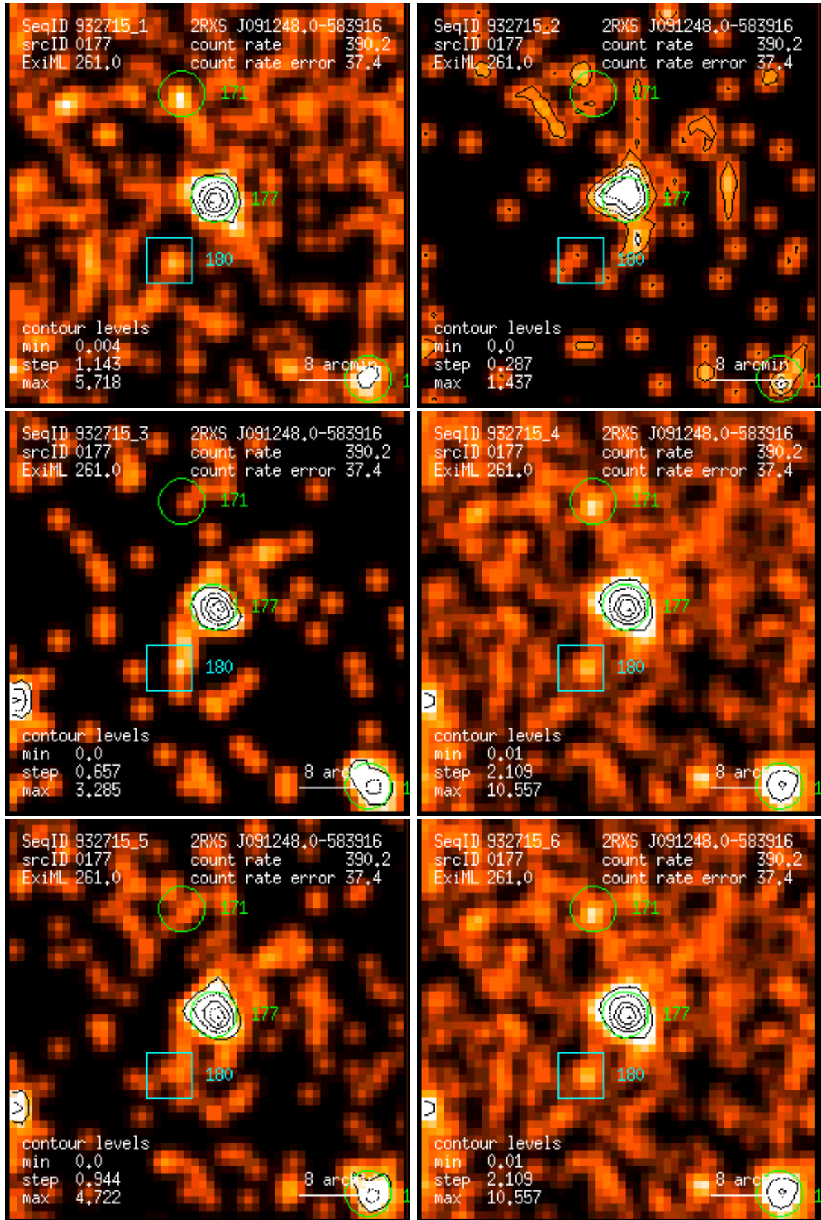
Figure 177: RASS 932715: detection 0177: band rate images, Gaussian filter: (1) PSPC channels 11 – 41, (2) 52 – 90, (3) 91 – 201, (4) 11 – 235, (5) 52 – 201, (6) 11 – 201. Broad band rates in counts/ks. Band rate contour levels in counts/ks/arcmin 2 .
