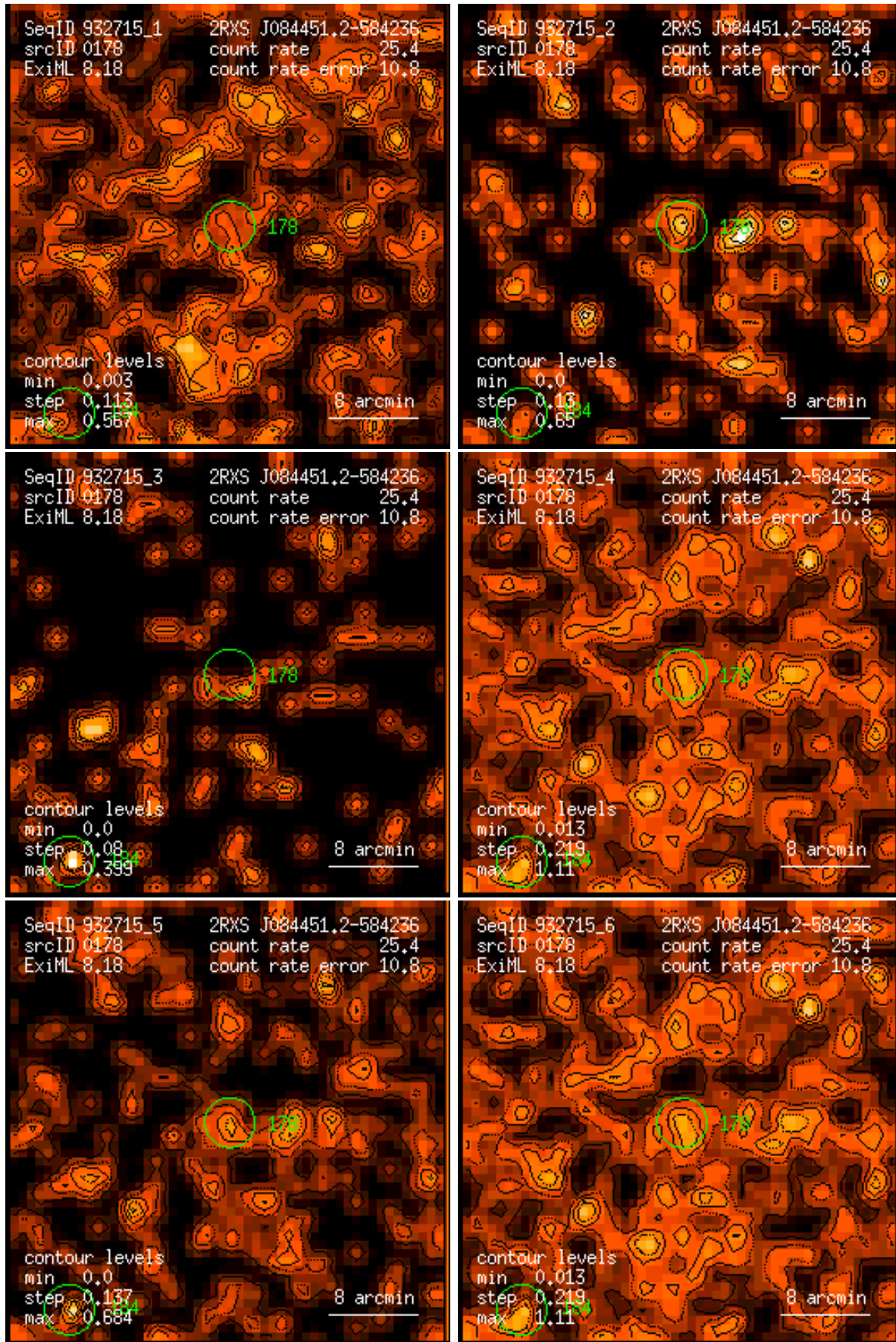
Figure 178: RASS 932715: detection 0178: band rate images, Gaussian filter: (1) PSPC channels 11 – 41, (2) 52 – 90, (3) 91 – 201, (4) 11 – 235, (5) 52 – 201, (6) 11 – 201. Broad band rates in counts/ks. Band rate contour levels in counts/ks/arcmin 2 .
