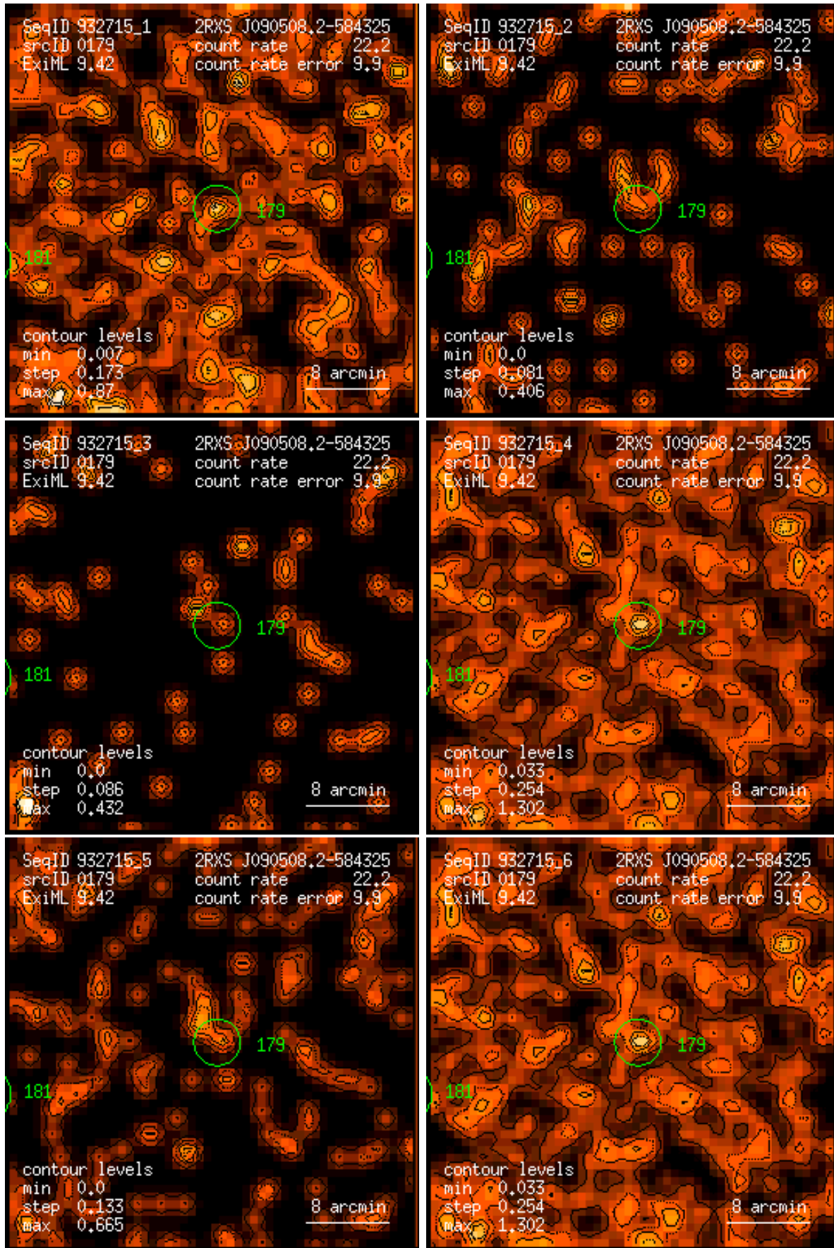
Figure 179: RASS 932715: detection 0179: band rate images, Gaussian filter: (1) PSPC channels 11 – 41, (2) 52 – 90, (3) 91 – 201, (4) 11 – 235, (5) 52 – 201, (6) 11 – 201. Broad band rates in counts/ks. Band rate contour levels in counts/ks/arcmin 2 .
