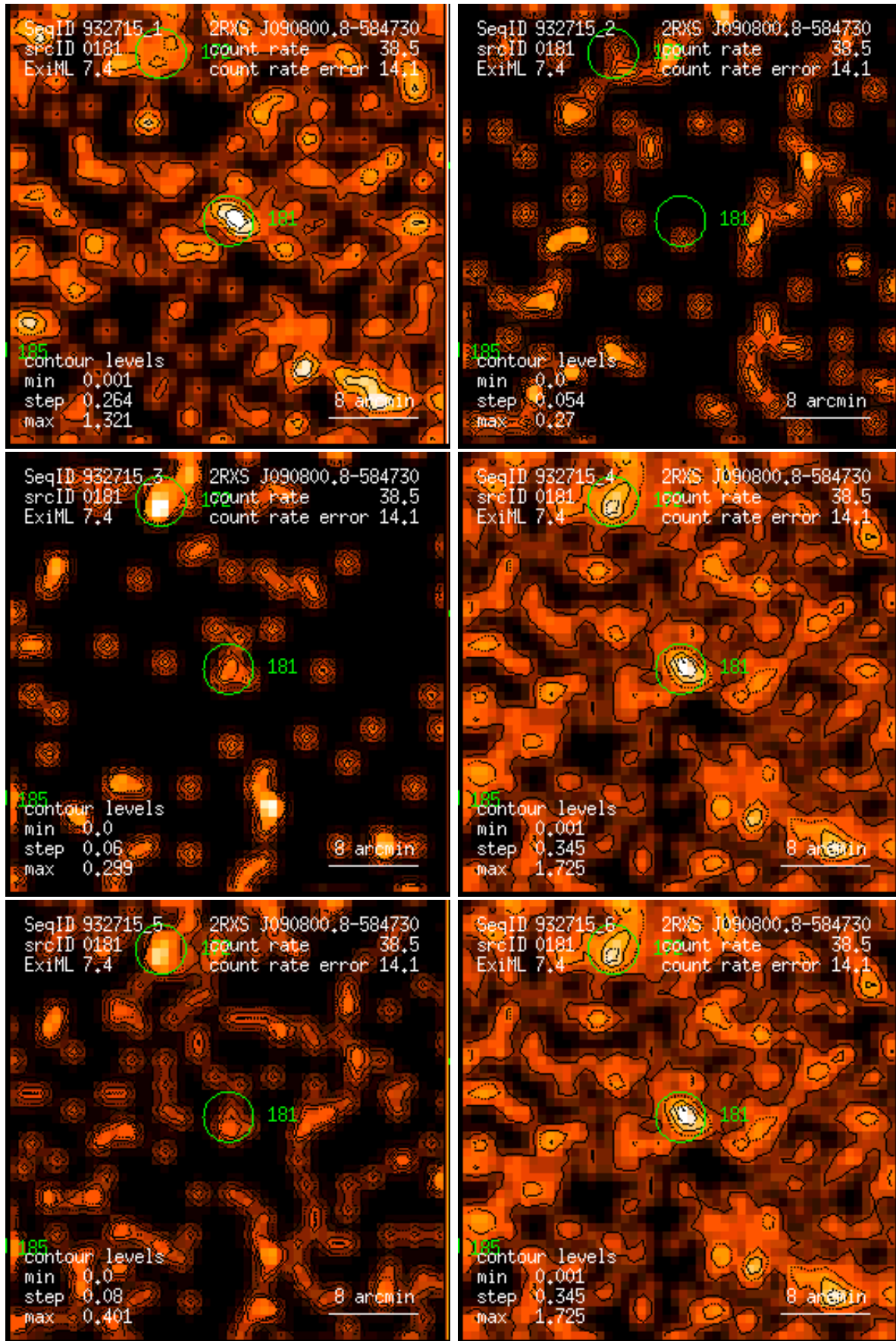
Figure 181: RASS 932715: detection 0181: band rate images, Gaussian filter: (1) PSPC channels 11 – 41, (2) 52 – 90, (3) 91 – 201, (4) 11 – 235, (5) 52 – 201, (6) 11 – 201. Broad band rates in counts/ks. Band rate contour levels in counts/ks/arcmin 2 .
