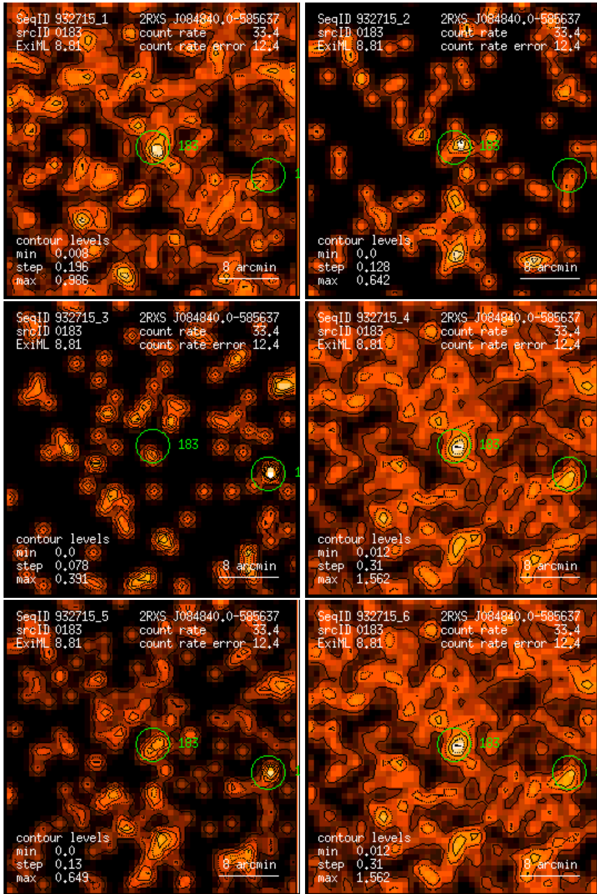
Figure 183: RASS 932715: detection 0183: band rate images, Gaussian filter: (1) PSPC channels 11 – 41, (2) 52 – 90, (3) 91 – 201, (4) 11 – 235, (5) 52 – 201, (6) 11 – 201. Broad band rates in counts/ks. Band rate contour levels in counts/ks/arcmin 2 .
