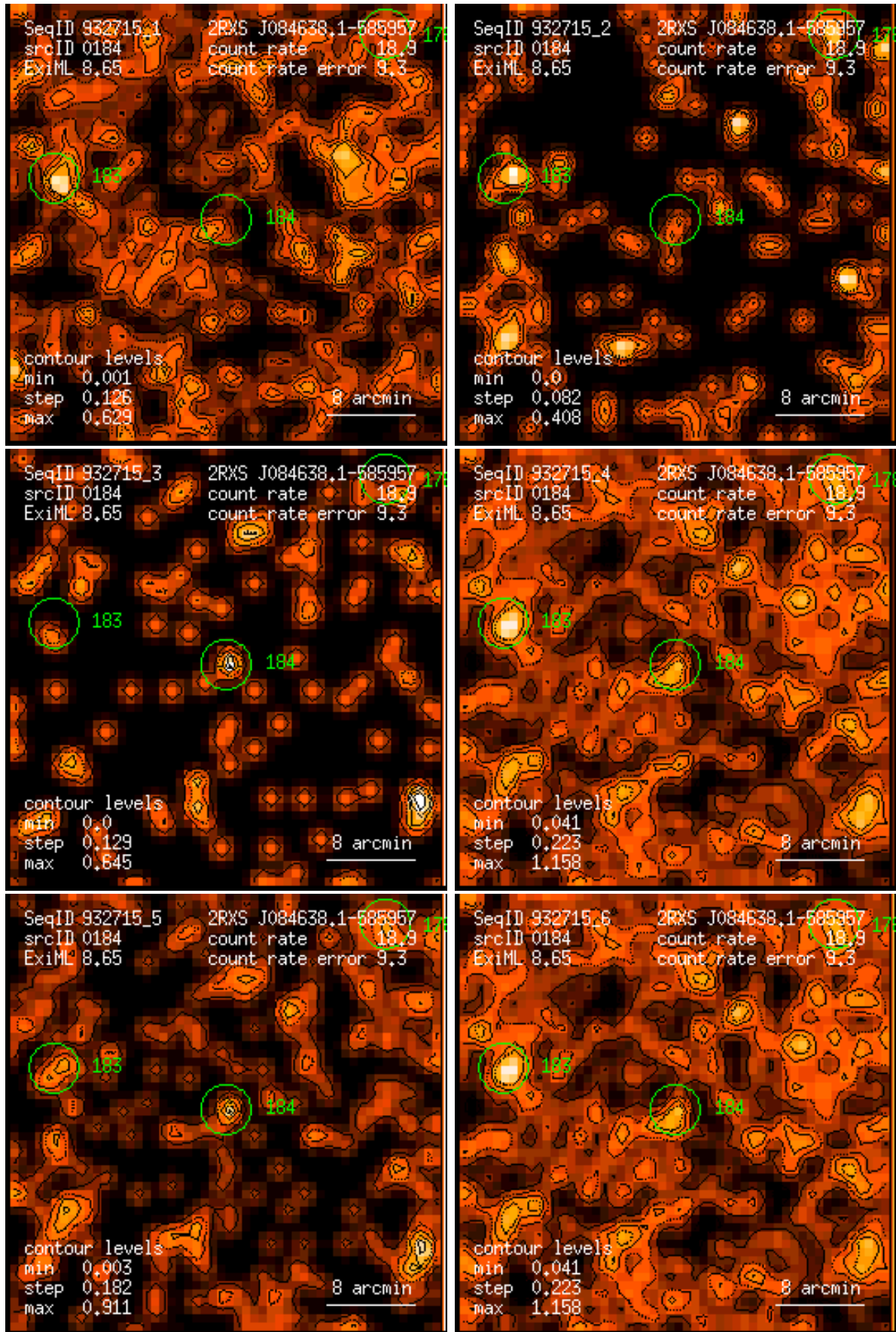
Figure 184: RASS 932715: detection 0184: band rate images, Gaussian filter: (1) PSPC channels 11 – 41, (2) 52 – 90, (3) 91 – 201, (4) 11 – 235, (5) 52 – 201, (6) 11 – 201. Broad band rates in counts/ks. Band rate contour levels in counts/ks/arcmin 2 .
