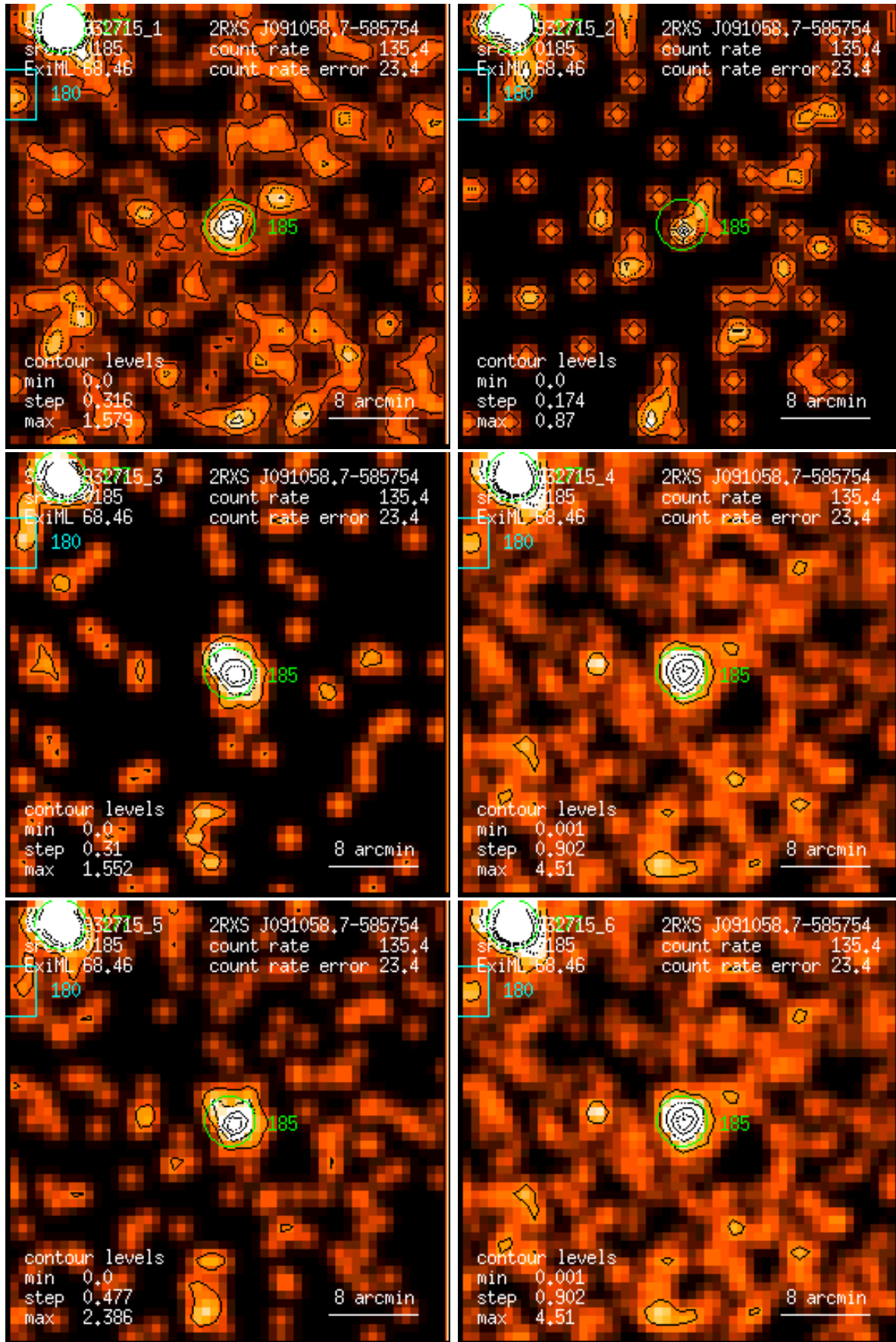
Figure 185: RASS 932715: detection 0185: band rate images, Gaussian filter: (1) PSPC channels 11 – 41, (2) 52 – 90, (3) 91 – 201, (4) 11 – 235, (5) 52 – 201, (6) 11 – 201. Broad band rates in counts/ks. Band rate contour levels in counts/ks/arcmin 2 .
