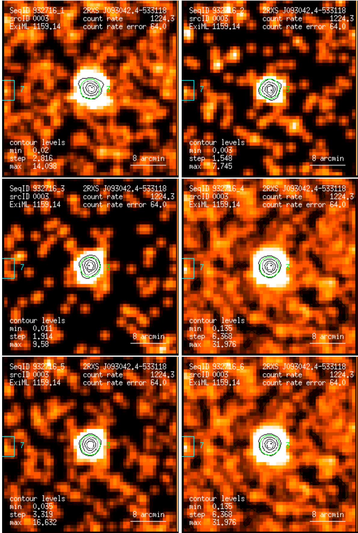
Figure 3: RASS 932716: detection 0003: band rate images, Gaussian filter: (1) PSPC channels 11 – 41, (2) 52 – 90, (3) 91 – 201, (4) 11 – 235, (5) 52 – 201, (6) 11 – 201. Broad band rates in counts/ks. Band rate contour levels in counts/ks/arcmin 2 .
