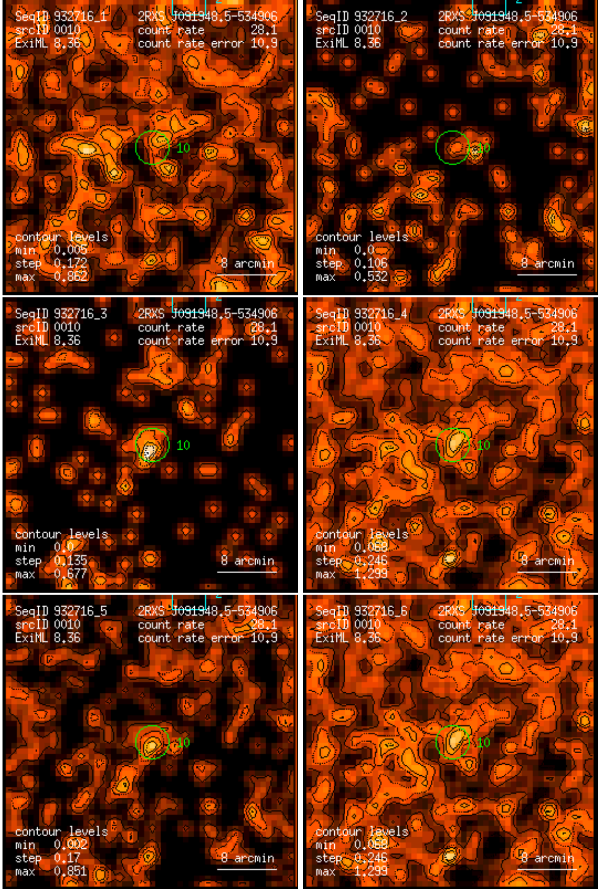
Figure 10: RASS 932716: detection 0010: band rate images, Gaussian filter: (1) PSPC channels 11 – 41, (2) 52 – 90, (3) 91 – 201, (4) 11 – 235, (5) 52 – 201, (6) 11 – 201. Broad band rates in counts/ks. Band rate contour levels in counts/ks/arcmin 2 .
