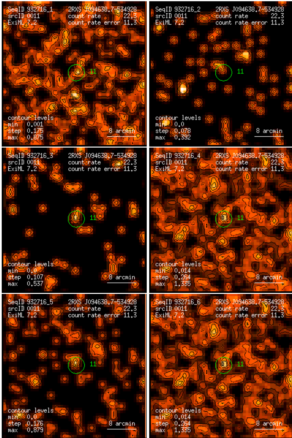
Figure 11: RASS 932716: detection 0011: band rate images, Gaussian filter: (1) PSPC channels 11 – 41, (2) 52 – 90, (3) 91 – 201, (4) 11 – 235, (5) 52 – 201, (6) 11 – 201. Broad band rates in counts/ks. Band rate contour levels in counts/ks/arcmin 2 .
