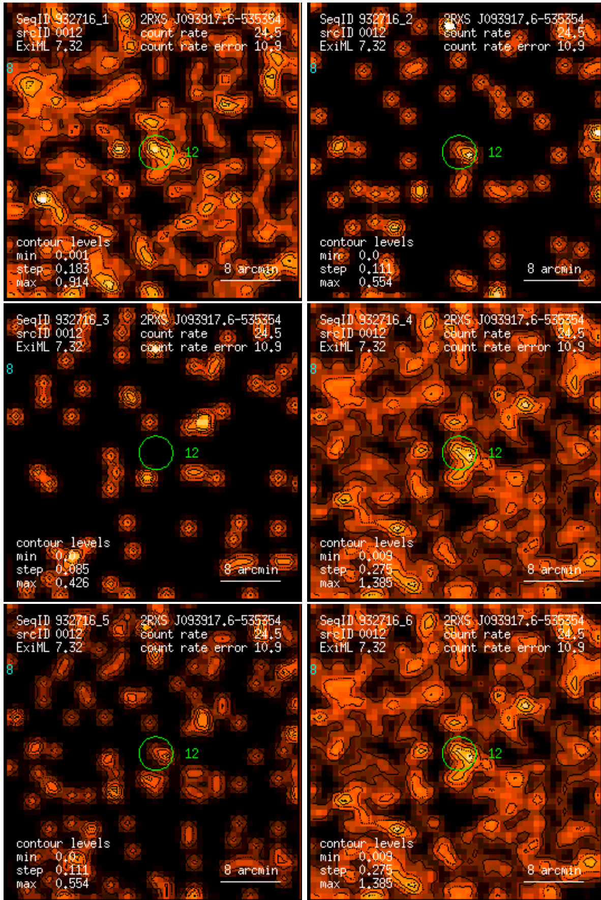
Figure 12: RASS 932716: detection 0012: band rate images, Gaussian filter: (1) PSPC channels 11 – 41, (2) 52 – 90, (3) 91 – 201, (4) 11 – 235, (5) 52 – 201, (6) 11 – 201. Broad band rates in counts/ks. Band rate contour levels in counts/ks/arcmin 2 .
