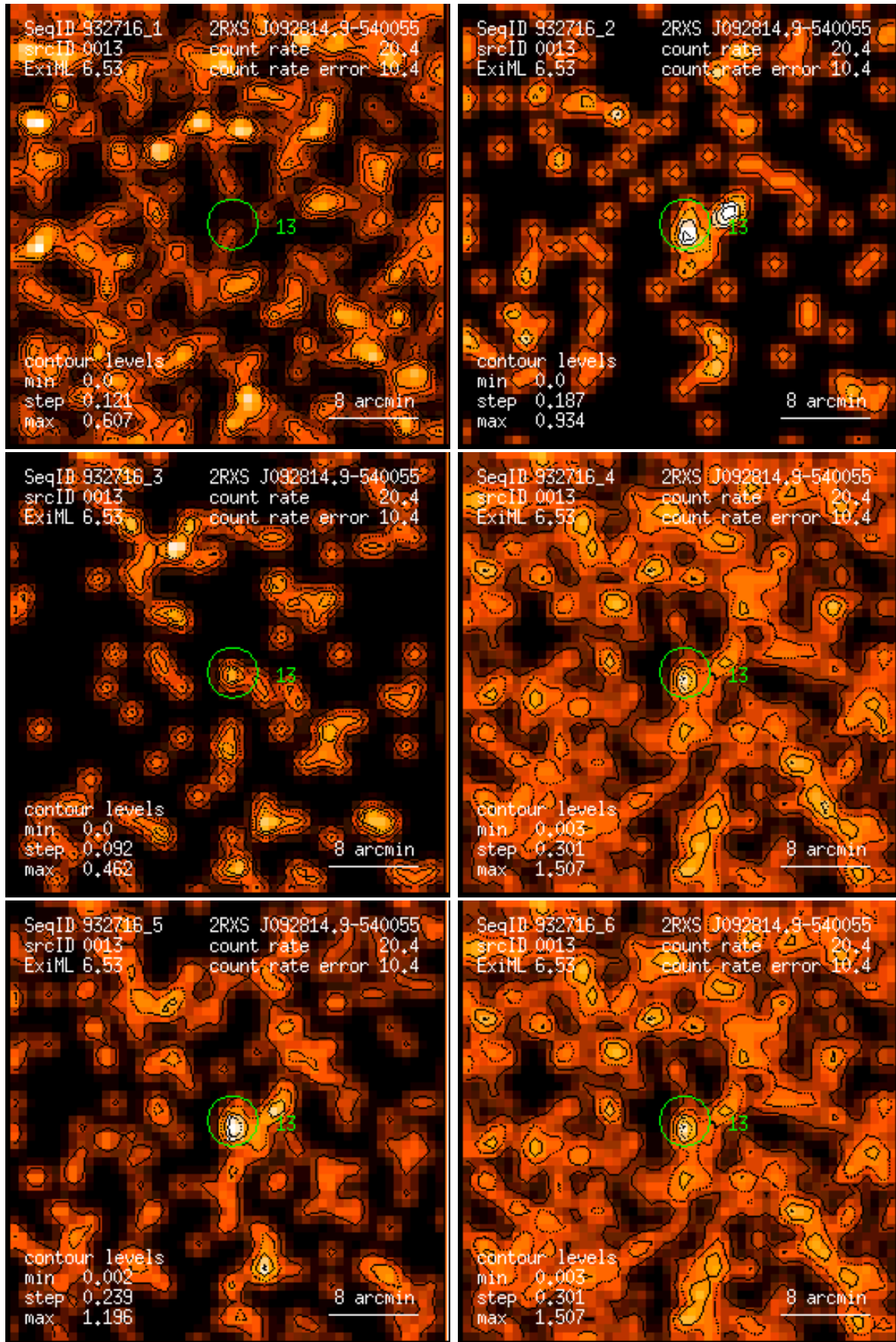
Figure 13: RASS 932716: detection 0013: band rate images, Gaussian filter: (1) PSPC channels 11 – 41, (2) 52 – 90, (3) 91 – 201, (4) 11 – 235, (5) 52 – 201, (6) 11 – 201. Broad band rates in counts/ks. Band rate contour levels in counts/ks/arcmin 2 .
