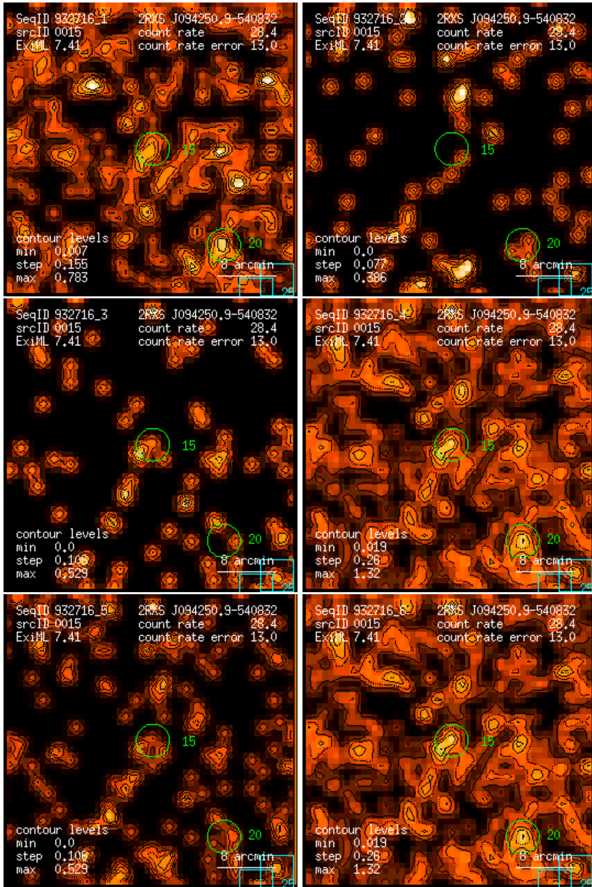
Figure 15: RASS 932716: detection 0015: band rate images, Gaussian filter: (1) PSPC channels 11 – 41, (2) 52 – 90, (3) 91 – 201, (4) 11 – 235, (5) 52 – 201, (6) 11 – 201. Broad band rates in counts/ks. Band rate contour levels in counts/ks/arcmin 2 .
