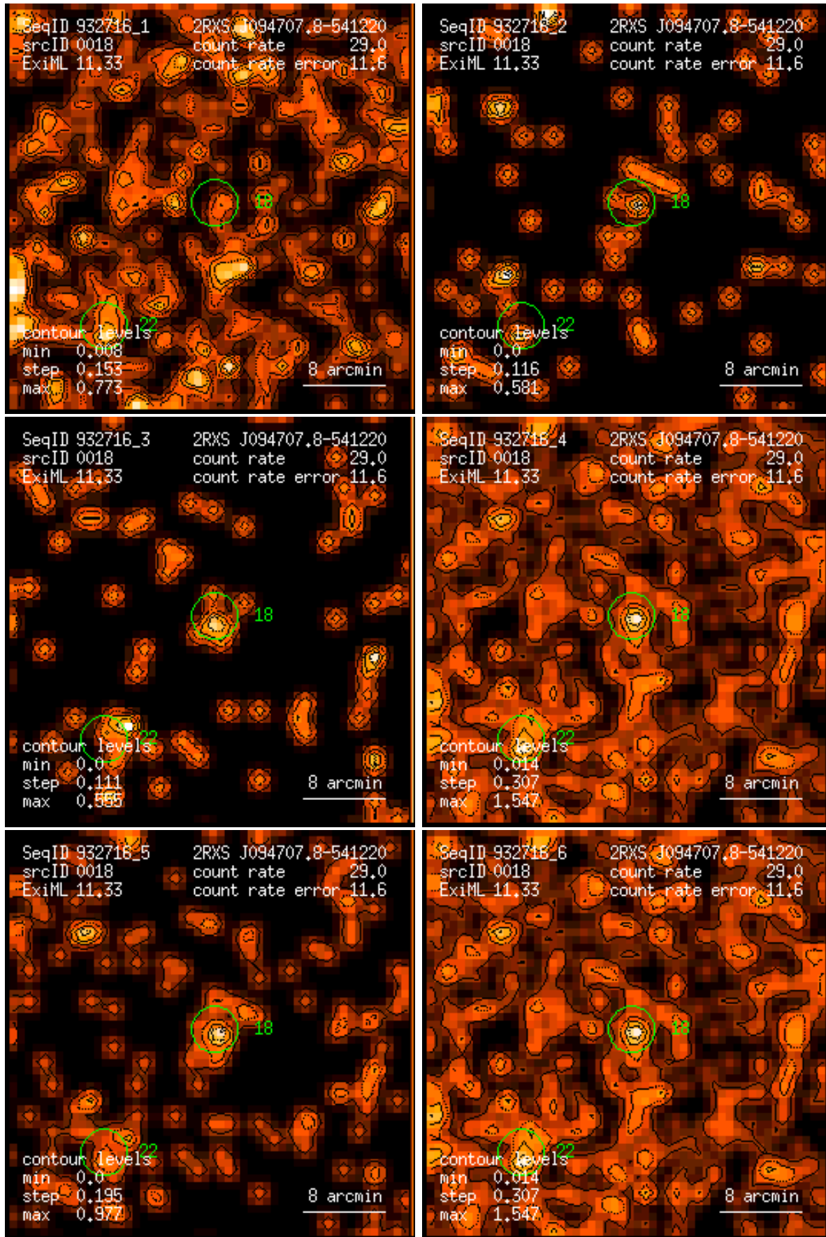
Figure 18: RASS 932716: detection 0018: band rate images, Gaussian filter: (1) PSPC channels 11 – 41, (2) 52 – 90, (3) 91 – 201, (4) 11 – 235, (5) 52 – 201, (6) 11 – 201. Broad band rates in counts/ks. Band rate contour levels in counts/ks/arcmin 2 .
