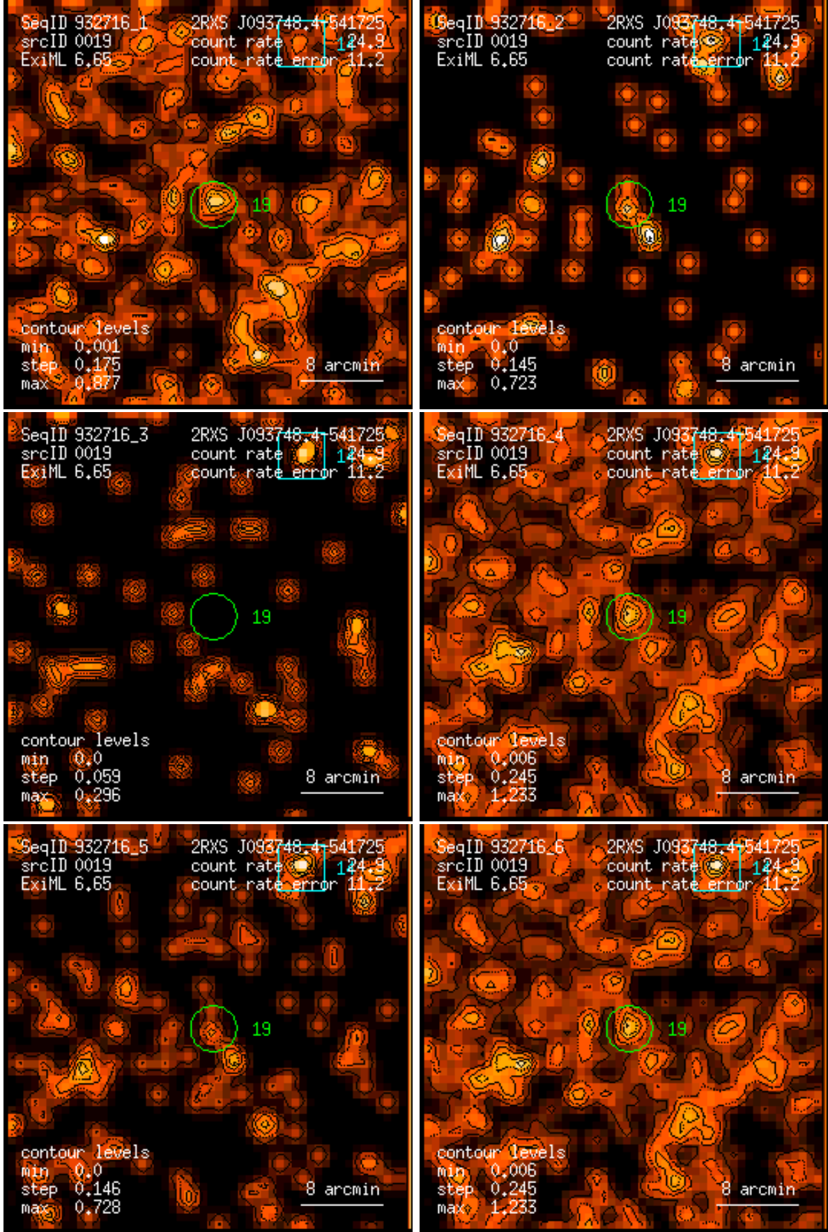
Figure 19: RASS 932716: detection 0019: band rate images, Gaussian filter: (1) PSPC channels 11 – 41, (2) 52 – 90, (3) 91 – 201, (4) 11 – 235, (5) 52 – 201, (6) 11 – 201. Broad band rates in counts/ks. Band rate contour levels in counts/ks/arcmin 2 .
