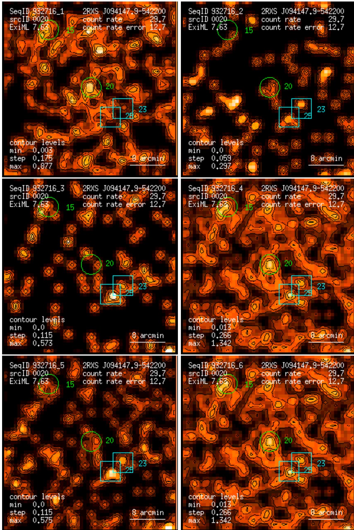
Figure 20: RASS 932716: detection 0020: band rate images, Gaussian filter: (1) PSPC channels 11 – 41, (2) 52 – 90, (3) 91 – 201, (4) 11 – 235, (5) 52 – 201, (6) 11 – 201. Broad band rates in counts/ks. Band rate contour levels in counts/ks/arcmin 2 .
