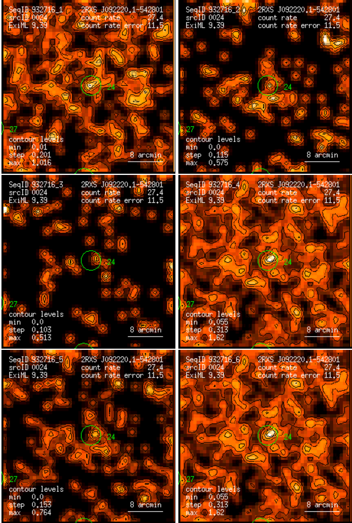
Figure 24: RASS 932716: detection 0024: band rate images, Gaussian filter: (1) PSPC channels 11 – 41, (2) 52 – 90, (3) 91 – 201, (4) 11 – 235, (5) 52 – 201, (6) 11 – 201. Broad band rates in counts/ks. Band rate contour levels in counts/ks/arcmin 2 .
