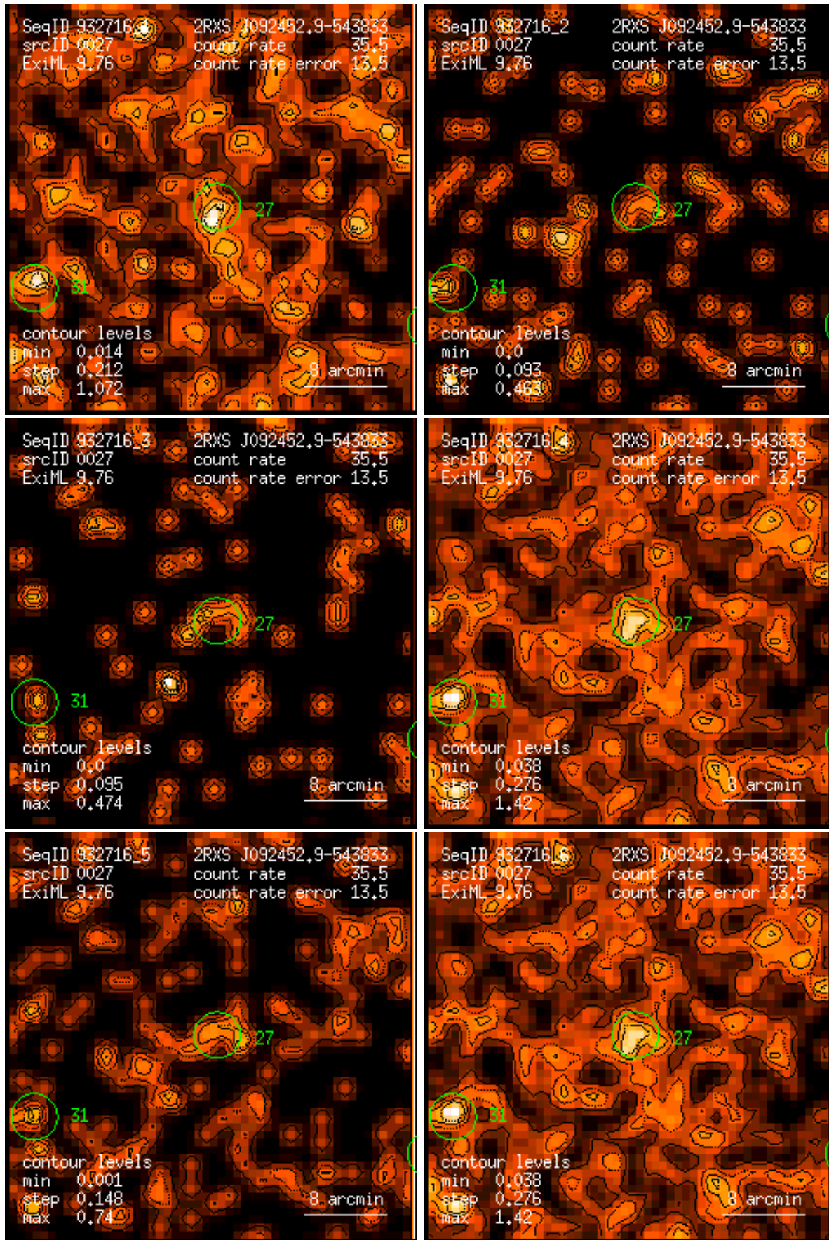
Figure 27: RASS 932716: detection 0027: band rate images, Gaussian filter: (1) PSPC channels 11 – 41, (2) 52 – 90, (3) 91 – 201, (4) 11 – 235, (5) 52 – 201, (6) 11 – 201. Broad band rates in counts/ks. Band rate contour levels in counts/ks/arcmin 2 .
