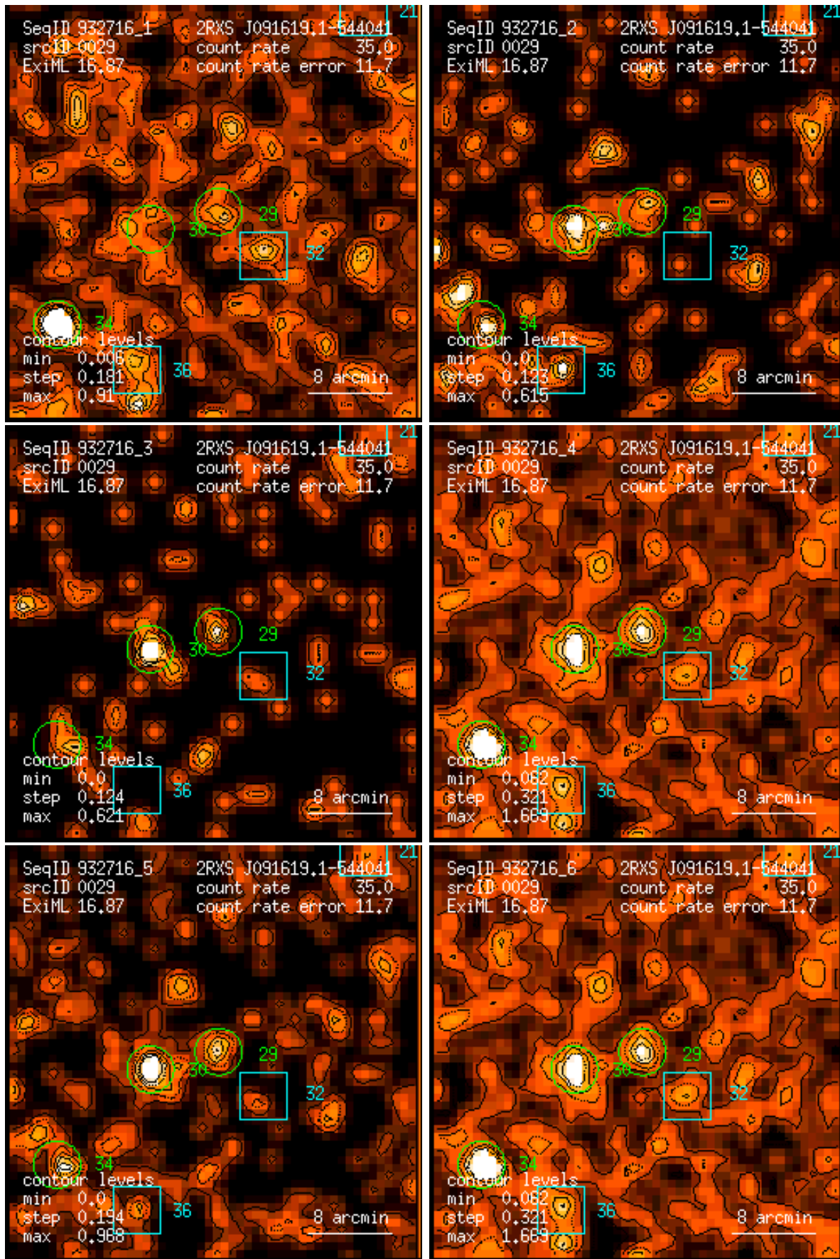
Figure 29: RASS 932716: detection 0029: band rate images, Gaussian filter: (1) PSPC channels 11 – 41, (2) 52 – 90, (3) 91 – 201, (4) 11 – 235, (5) 52 – 201, (6) 11 – 201. Broad band rates in counts/ks. Band rate contour levels in counts/ks/arcmin 2 .
