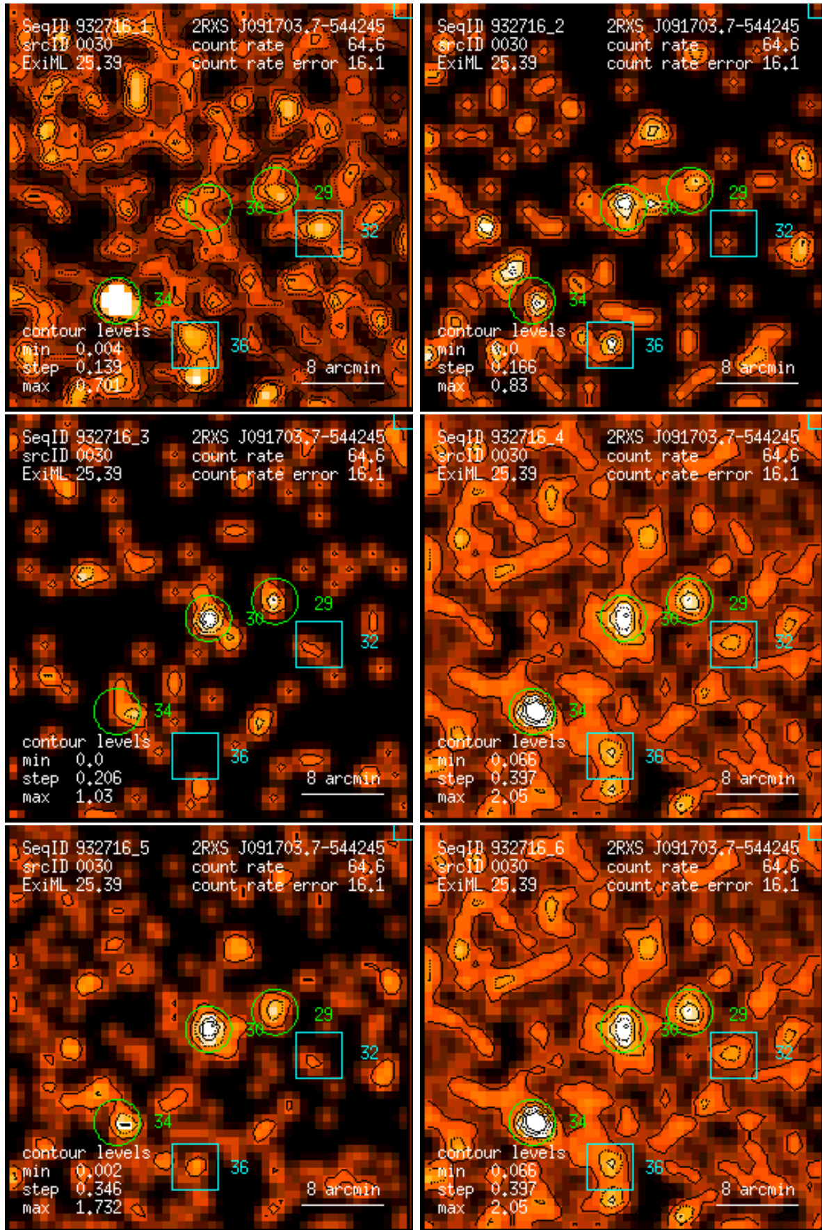
Figure 30: RASS 932716: detection 0030: band rate images, Gaussian filter: (1) PSPC channels 11 – 41, (2) 52 – 90, (3) 91 – 201, (4) 11 – 235, (5) 52 – 201, (6) 11 – 201. Broad band rates in counts/ks. Band rate contour levels in counts/ks/arcmin 2 .
