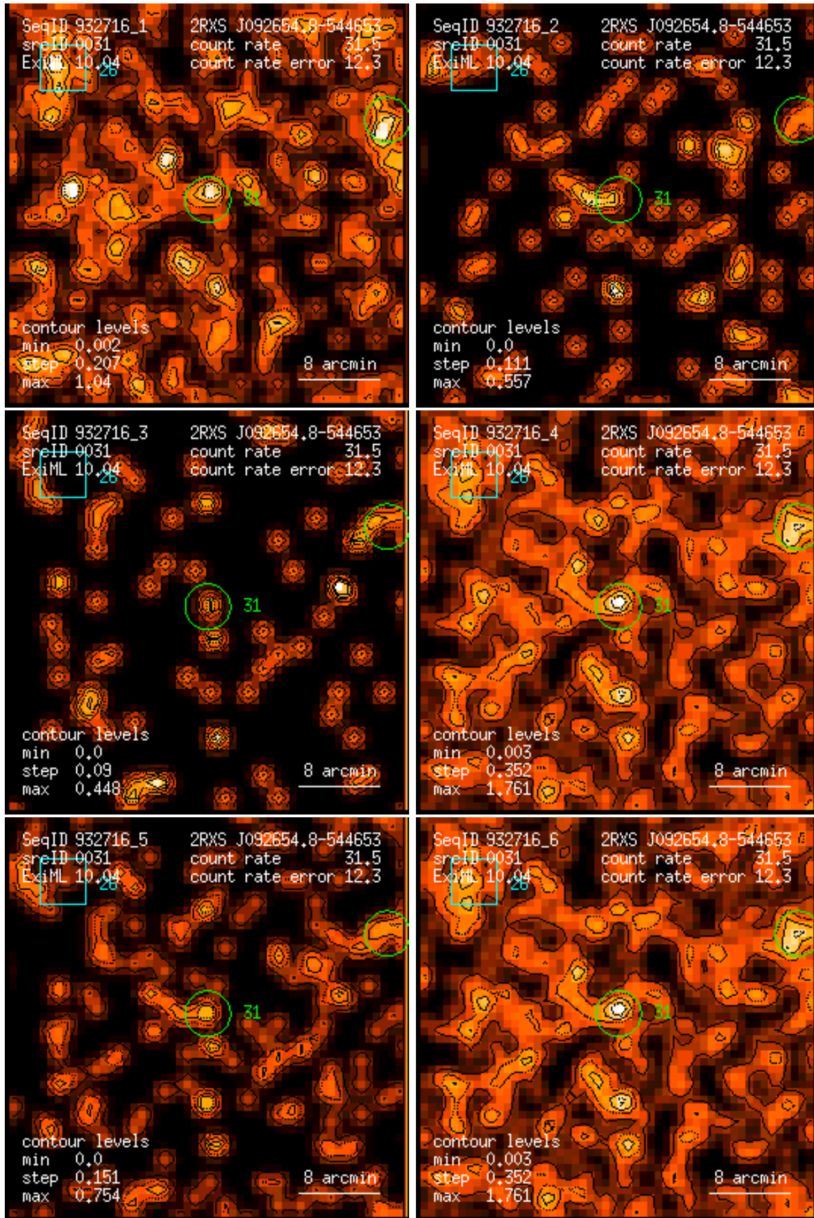
Figure 31: RASS 932716: detection 0031: band rate images, Gaussian filter: (1) PSPC channels 11 – 41, (2) 52 – 90, (3) 91 – 201, (4) 11 – 235, (5) 52 – 201, (6) 11 – 201. Broad band rates in counts/ks. Band rate contour levels in counts/ks/arcmin 2 .
