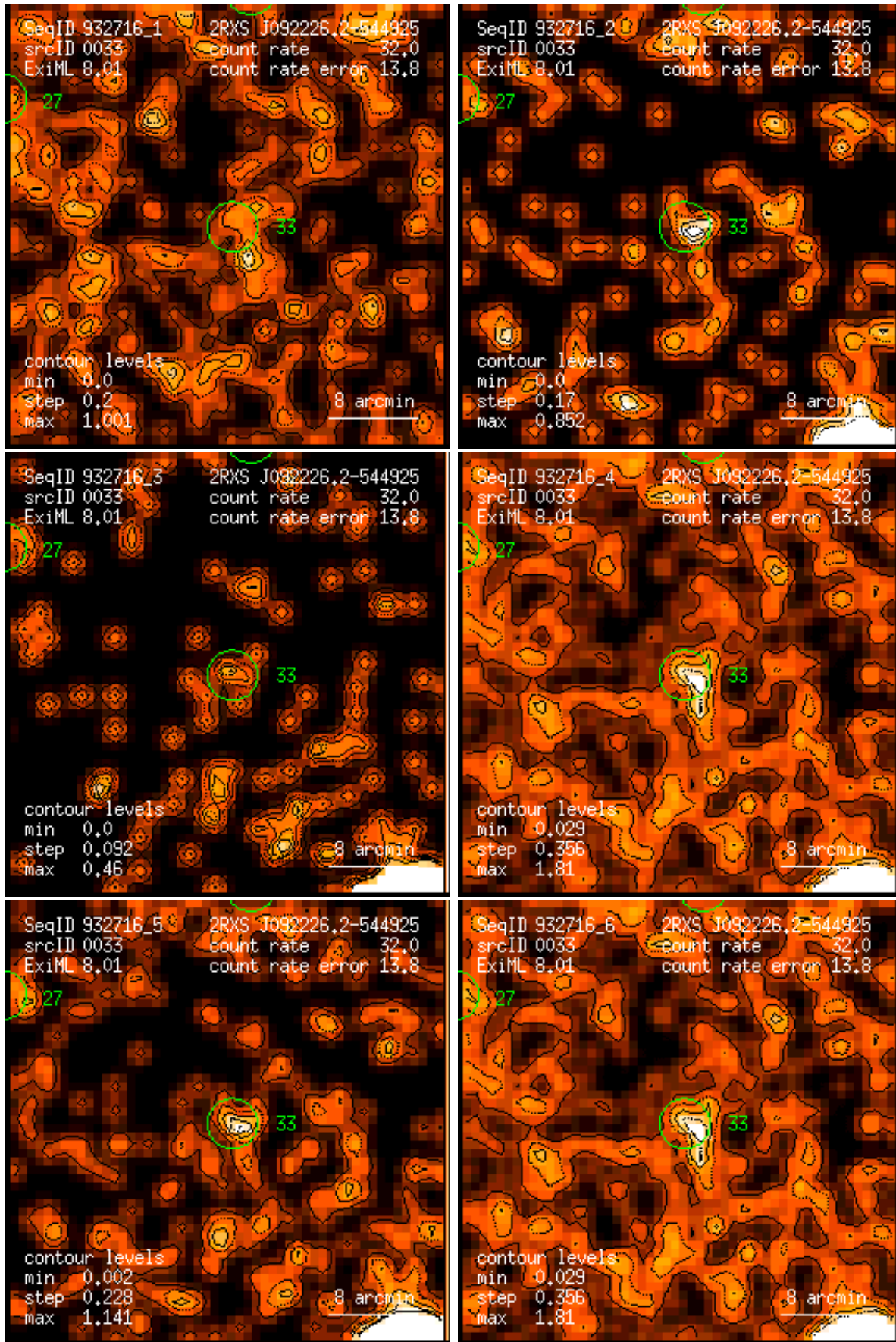
Figure 33: RASS 932716: detection 0033: band rate images, Gaussian filter: (1) PSPC channels 11 – 41, (2) 52 – 90, (3) 91 – 201, (4) 11 – 235, (5) 52 – 201, (6) 11 – 201. Broad band rates in counts/ks. Band rate contour levels in counts/ks/arcmin 2 .
