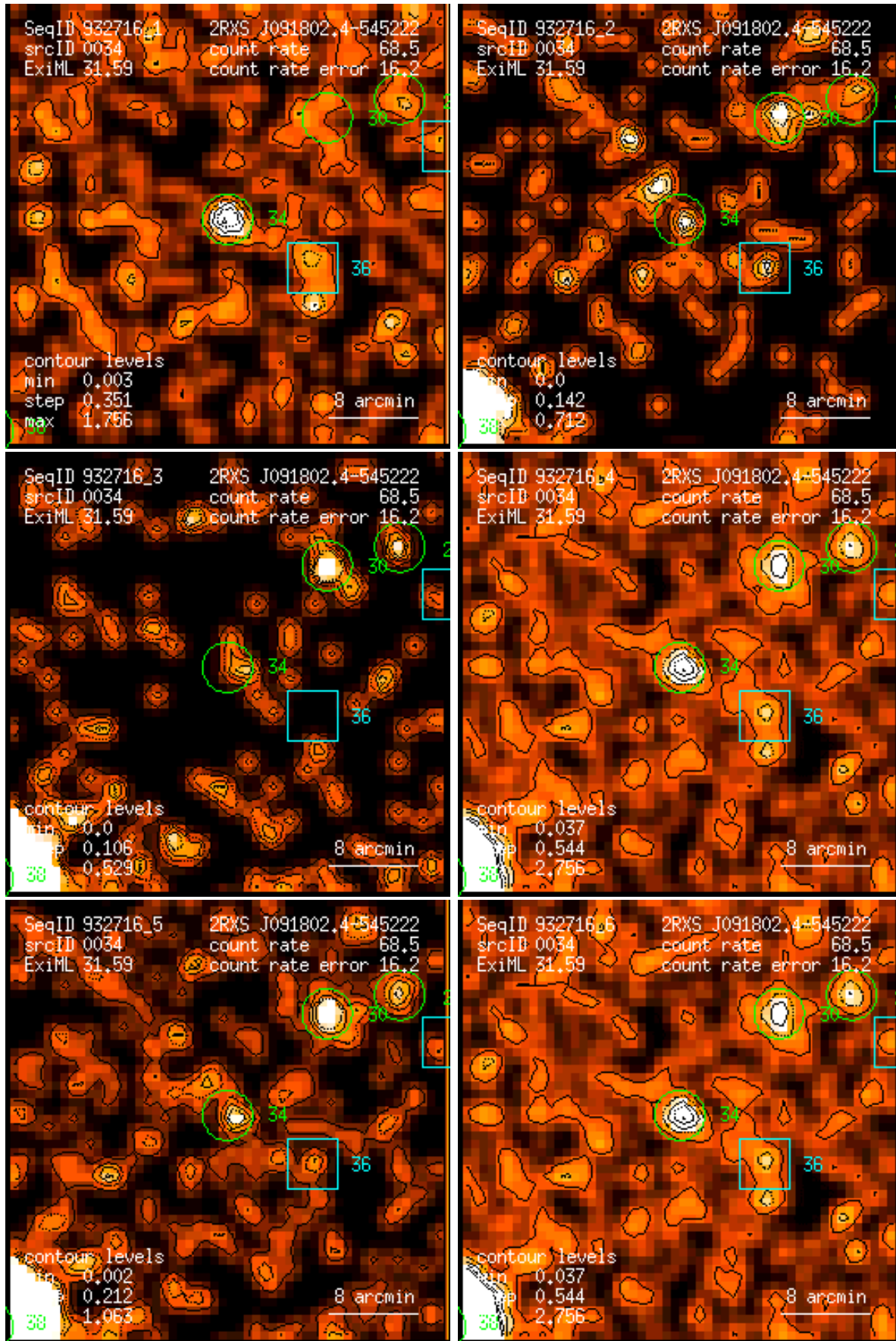
Figure 34: RASS 932716: detection 0034: band rate images, Gaussian filter: (1) PSPC channels 11 – 41, (2) 52 – 90, (3) 91 – 201, (4) 11 – 235, (5) 52 – 201, (6) 11 – 201. Broad band rates in counts/ks. Band rate contour levels in counts/ks/arcmin 2 .
