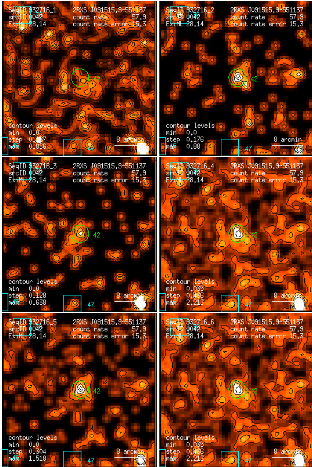
Figure 42: RASS 932716: detection 0042: band rate images, Gaussian filter: (1) PSPC channels 11 – 41, (2) 52 – 90, (3) 91 – 201, (4) 11 – 235, (5) 52 – 201, (6) 11 – 201. Broad band rates in counts/ks. Band rate contour levels in counts/ks/arcmin 2 .
