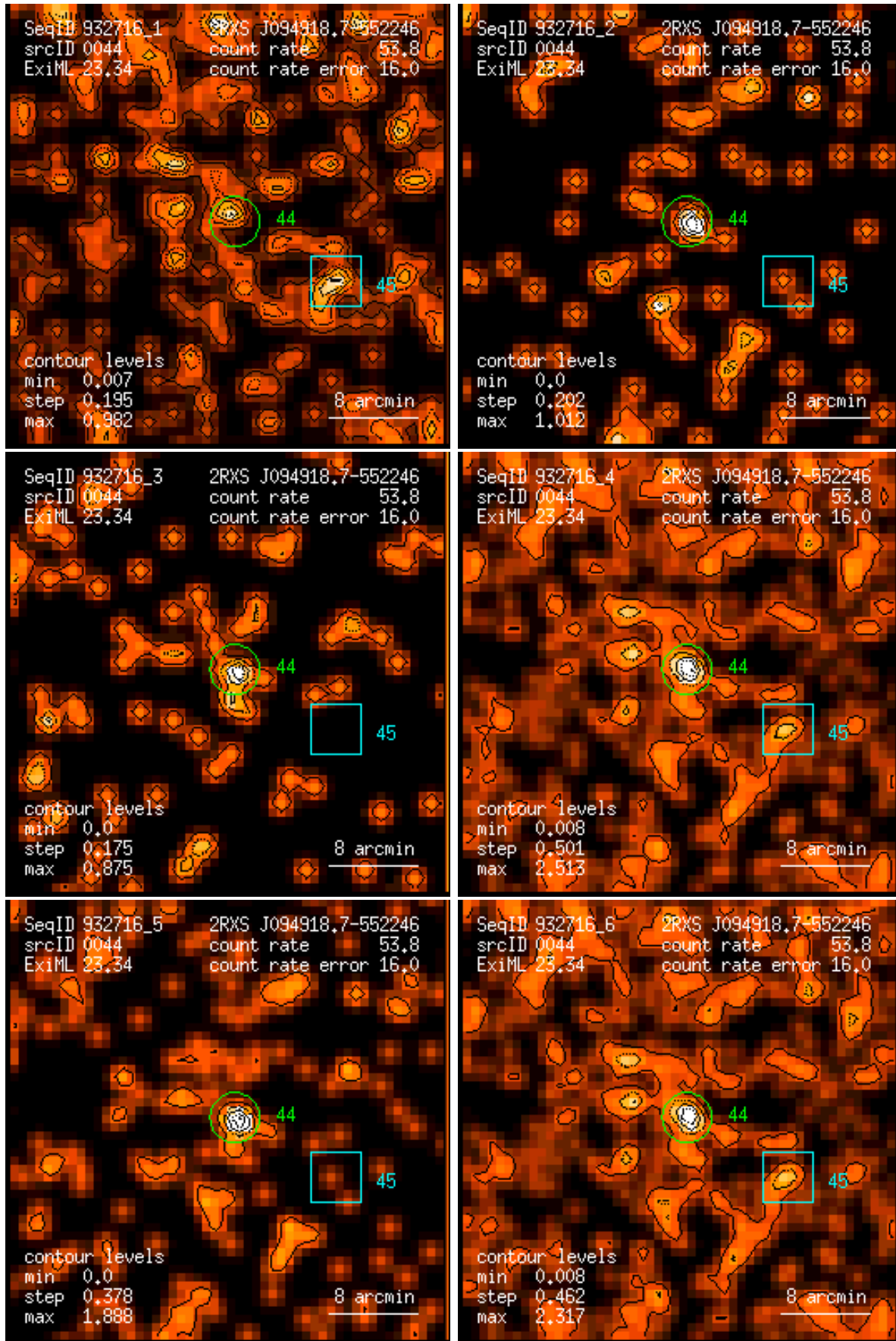
Figure 44: RASS 932716: detection 0044: band rate images, Gaussian filter: (1) PSPC channels 11 – 41, (2) 52 – 90, (3) 91 – 201, (4) 11 – 235, (5) 52 – 201, (6) 11 – 201. Broad band rates in counts/ks. Band rate contour levels in counts/ks/arcmin 2 .
