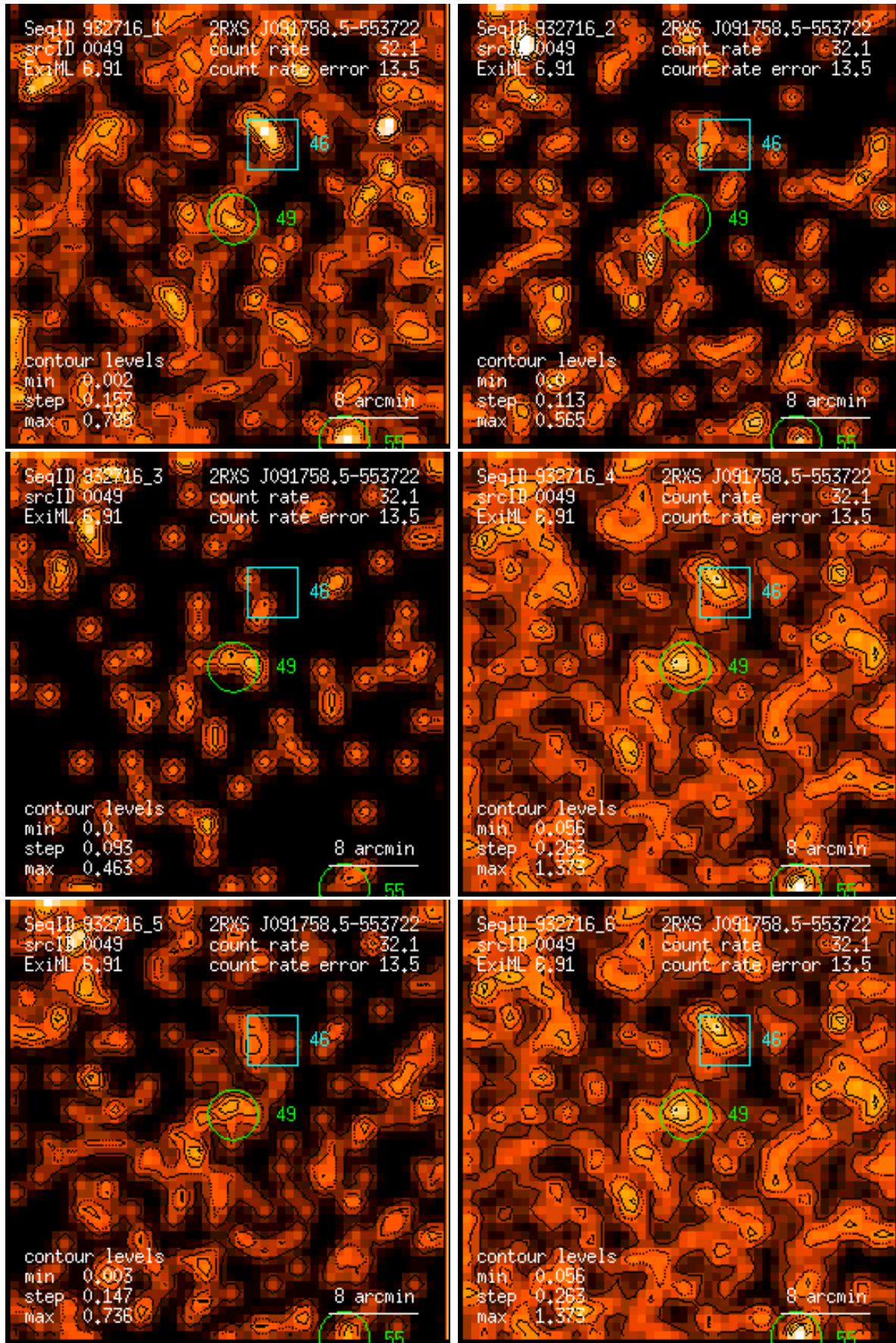
Figure 49: RASS 932716: detection 0049: band rate images, Gaussian filter: (1) PSPC channels 11 – 41, (2) 52 – 90, (3) 91 – 201, (4) 11 – 235, (5) 52 – 201, (6) 11 – 201. Broad band rates in counts/ks. Band rate contour levels in counts/ks/arcmin 2 .
