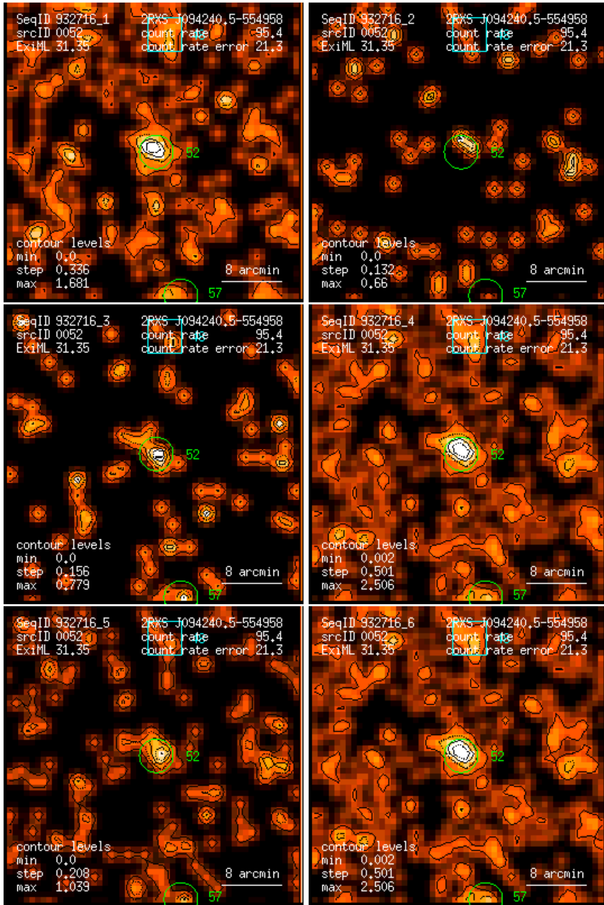
Figure 52: RASS 932716: detection 0052: band rate images, Gaussian filter: (1) PSPC channels 11 – 41, (2) 52 – 90, (3) 91 – 201, (4) 11 – 235, (5) 52 – 201, (6) 11 – 201. Broad band rates in counts/ks. Band rate contour levels in counts/ks/arcmin 2 .
