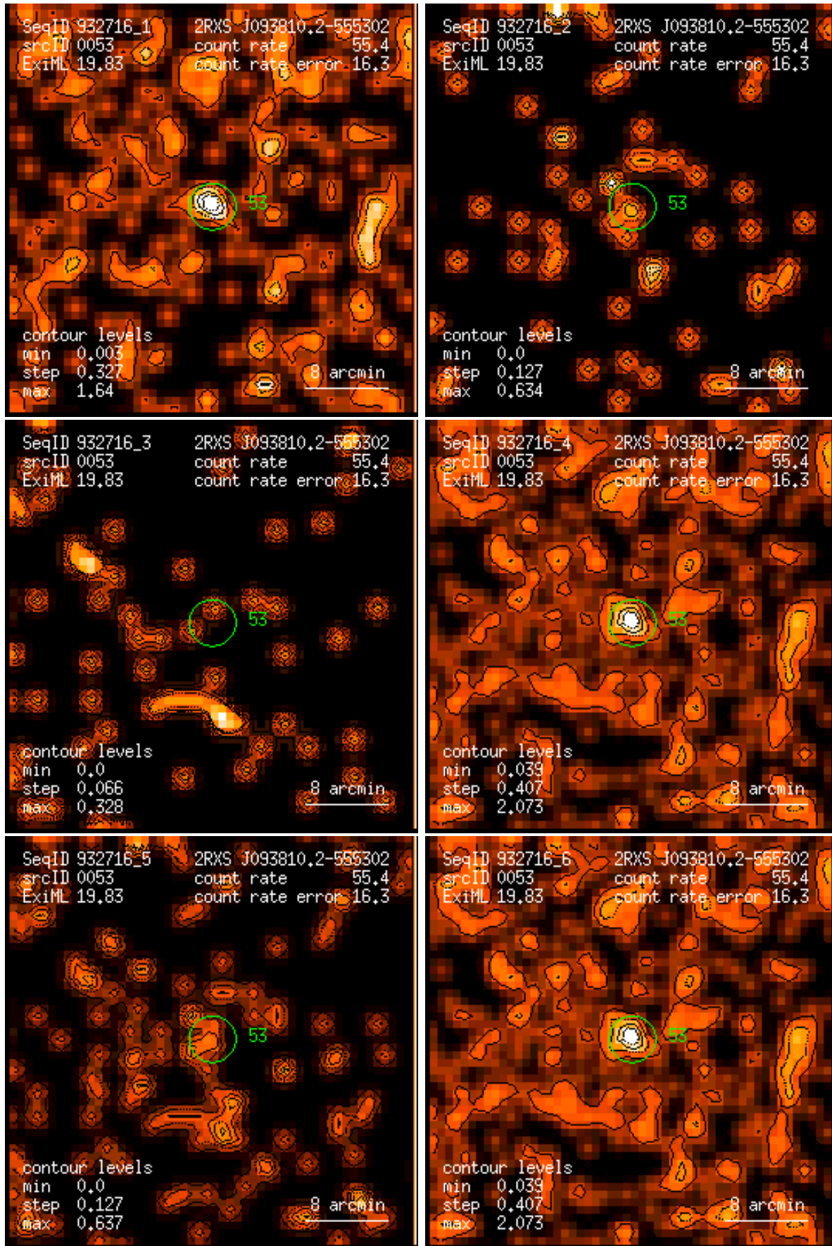
Figure 53: RASS 932716: detection 0053: band rate images, Gaussian filter: (1) PSPC channels 11 – 41, (2) 52 – 90, (3) 91 – 201, (4) 11 – 235, (5) 52 – 201, (6) 11 – 201. Broad band rates in counts/ks. Band rate contour levels in counts/ks/arcmin 2 .
