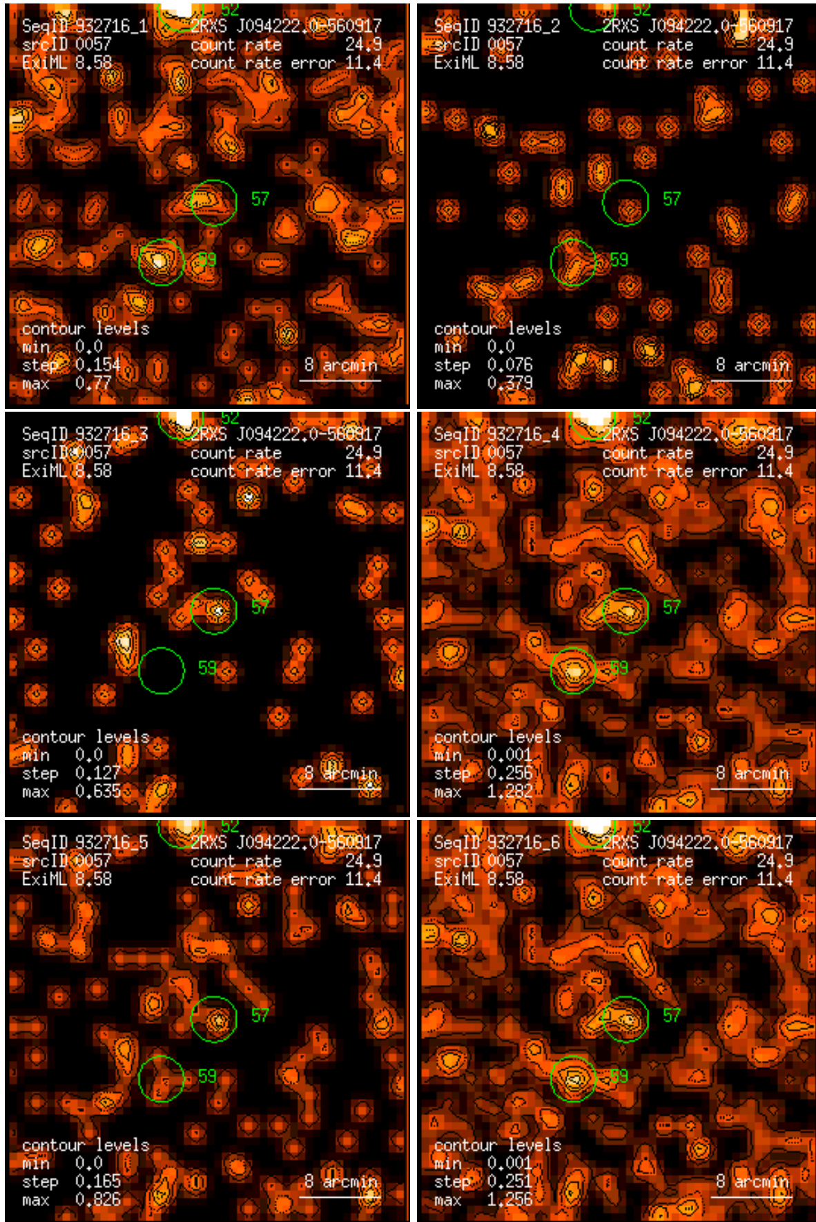
Figure 57: RASS 932716: detection 0057: band rate images, Gaussian filter: (1) PSPC channels 11 – 41, (2) 52 – 90, (3) 91 – 201, (4) 11 – 235, (5) 52 – 201, (6) 11 – 201. Broad band rates in counts/ks. Band rate contour levels in counts/ks/arcmin 2 .
