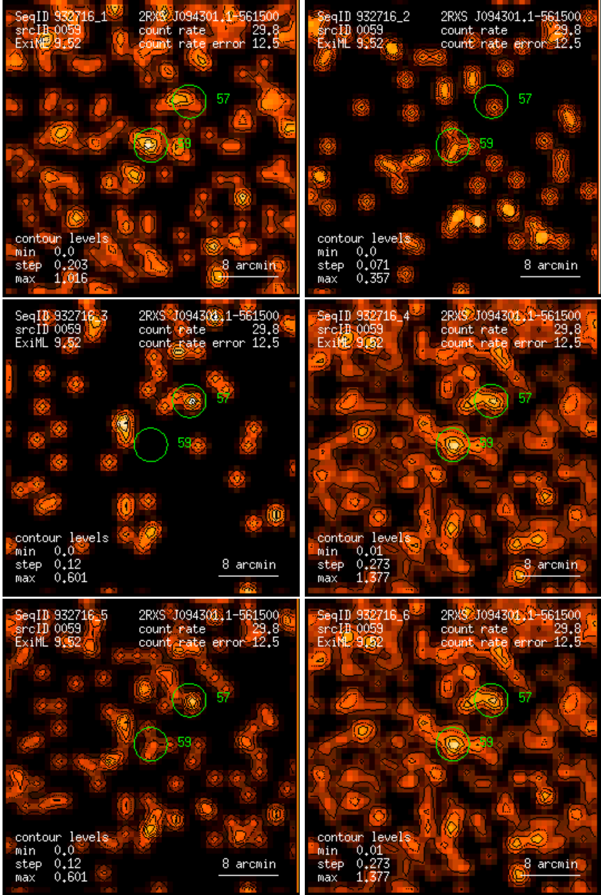
Figure 59: RASS 932716: detection 0059: band rate images, Gaussian filter: (1) PSPC channels 11 – 41, (2) 52 – 90, (3) 91 – 201, (4) 11 – 235, (5) 52 – 201, (6) 11 – 201. Broad band rates in counts/ks. Band rate contour levels in counts/ks/arcmin 2 .
