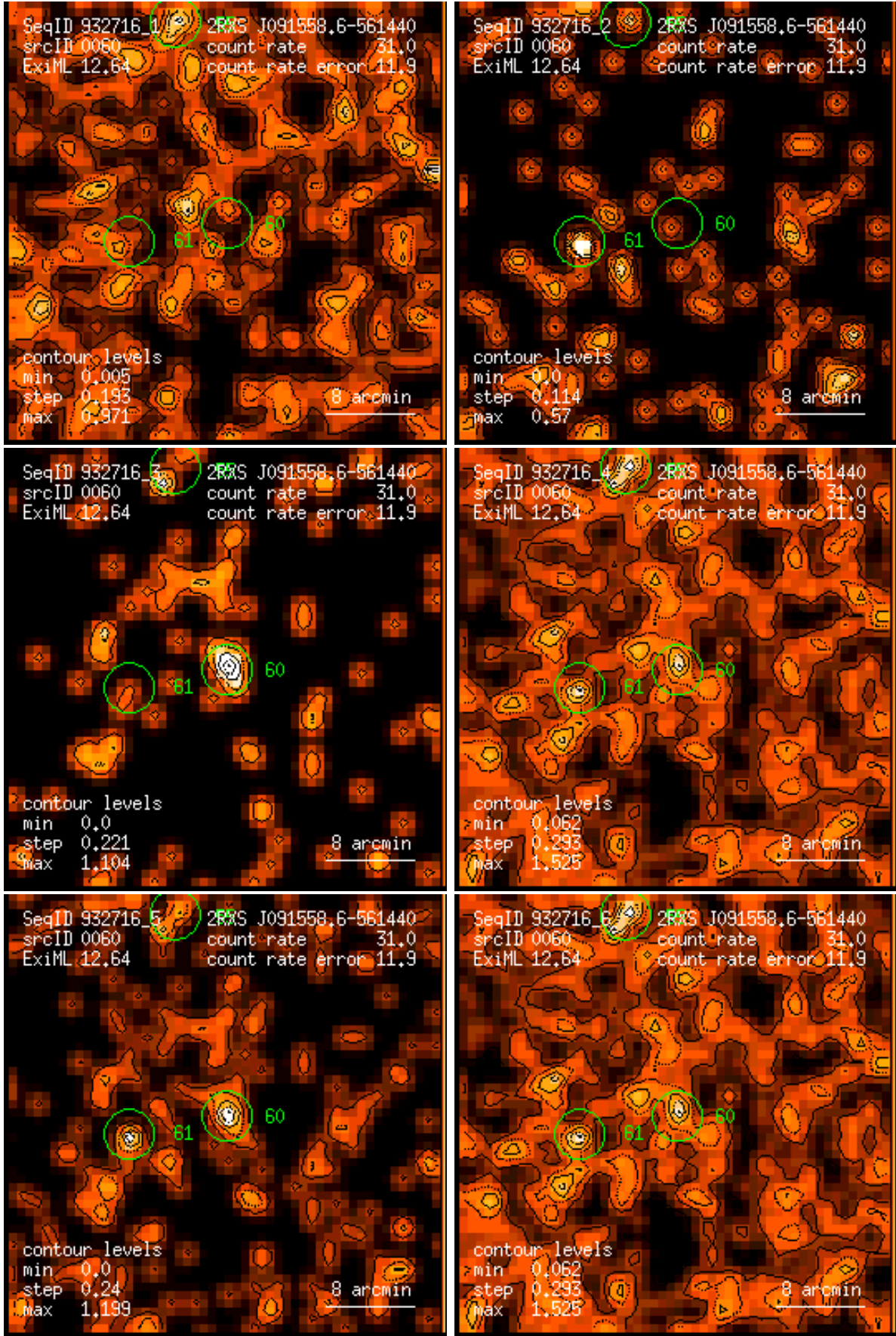
Figure 60: RASS 932716: detection 0060: band rate images, Gaussian filter: (1) PSPC channels 11 – 41, (2) 52 – 90, (3) 91 – 201, (4) 11 – 235, (5) 52 – 201, (6) 11 – 201. Broad band rates in counts/ks. Band rate contour levels in counts/ks/arcmin 2 .
