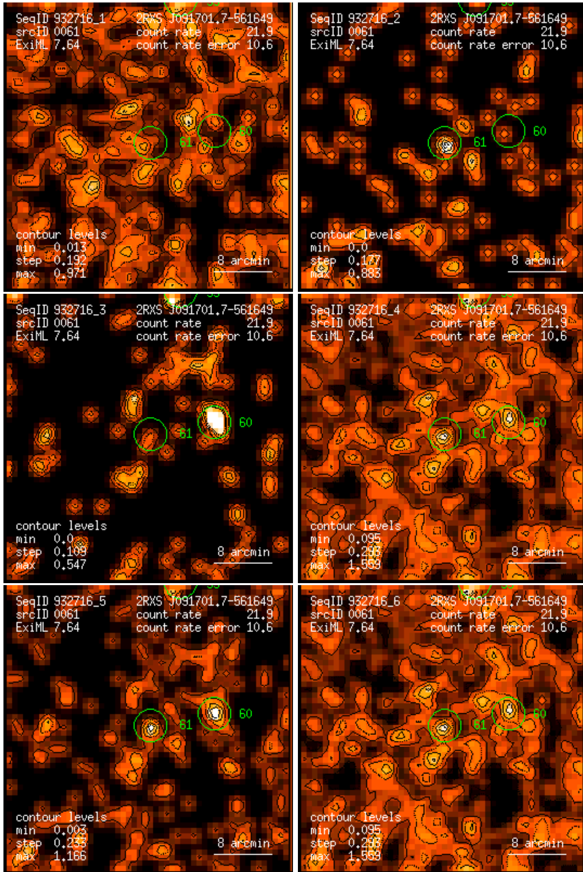
Figure 61: RASS 932716: detection 0061: band rate images, Gaussian filter: (1) PSPC channels 11 – 41, (2) 52 – 90, (3) 91 – 201, (4) 11 – 235, (5) 52 – 201, (6) 11 – 201. Broad band rates in counts/ks. Band rate contour levels in counts/ks/arcmin 2 .
