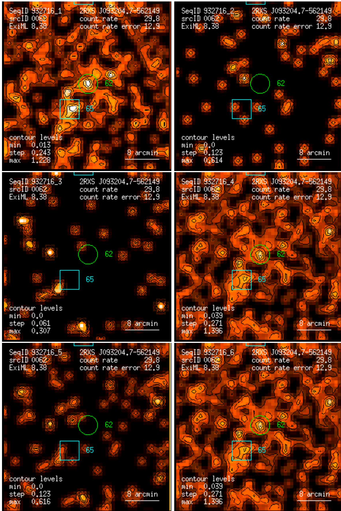
Figure 62: RASS 932716: detection 0062: band rate images, Gaussian filter: (1) PSPC channels 11 – 41, (2) 52 – 90, (3) 91 – 201, (4) 11 – 235, (5) 52 – 201, (6) 11 – 201. Broad band rates in counts/ks. Band rate contour levels in counts/ks/arcmin 2 .
