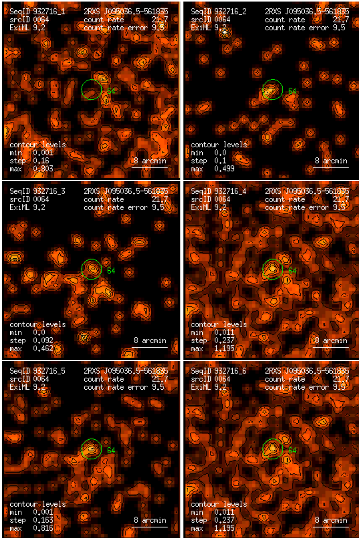
Figure 64: RASS 932716: detection 0064: band rate images, Gaussian filter: (1) PSPC channels 11 – 41, (2) 52 – 90, (3) 91 – 201, (4) 11 – 235, (5) 52 – 201, (6) 11 – 201. Broad band rates in counts/ks. Band rate contour levels in counts/ks/arcmin 2 .
