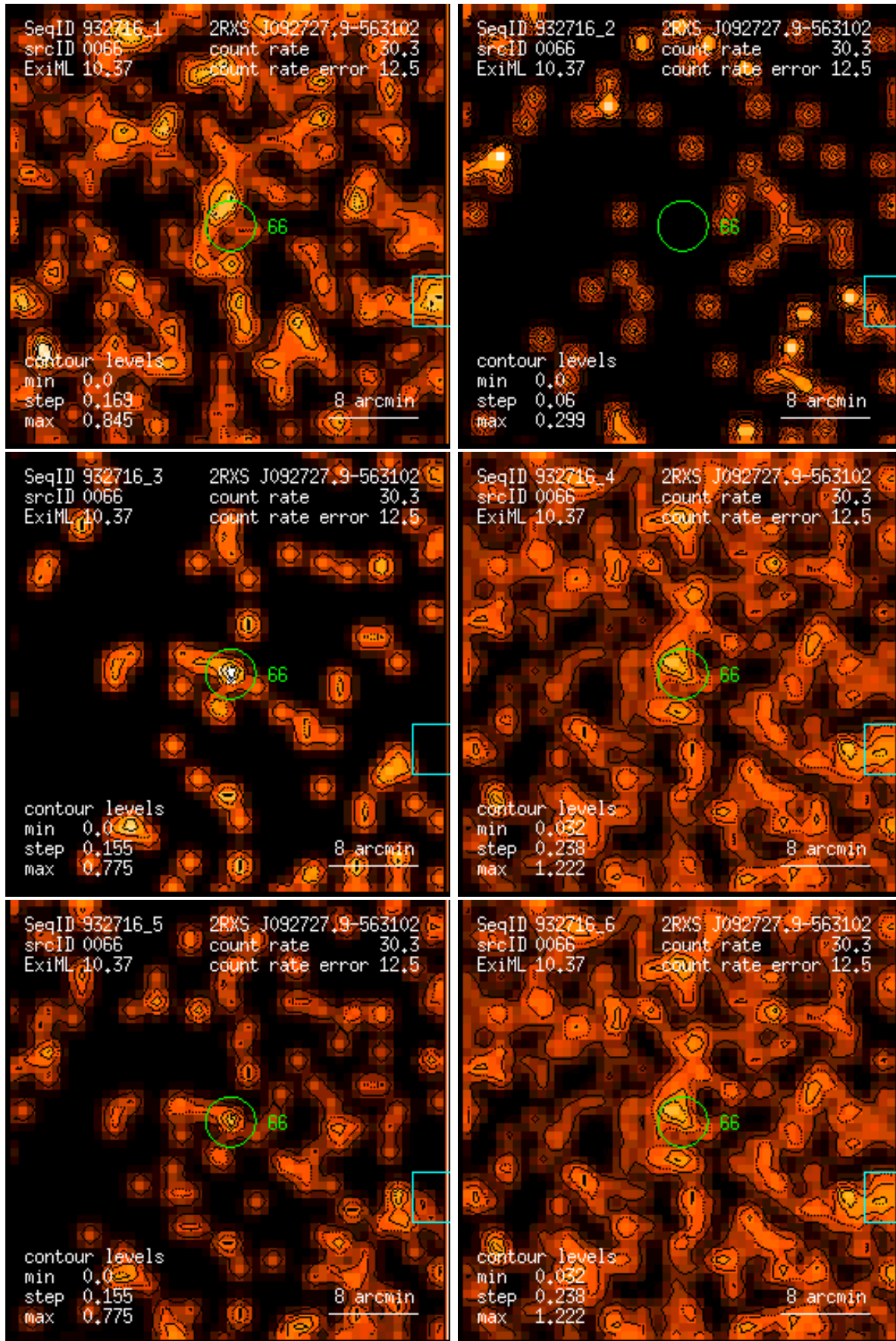
Figure 66: RASS 932716: detection 0066: band rate images, Gaussian filter: (1) PSPC channels 11 – 41, (2) 52 – 90, (3) 91 – 201, (4) 11 – 235, (5) 52 – 201, (6) 11 – 201. Broad band rates in counts/ks. Band rate contour levels in counts/ks/arcmin 2 .
