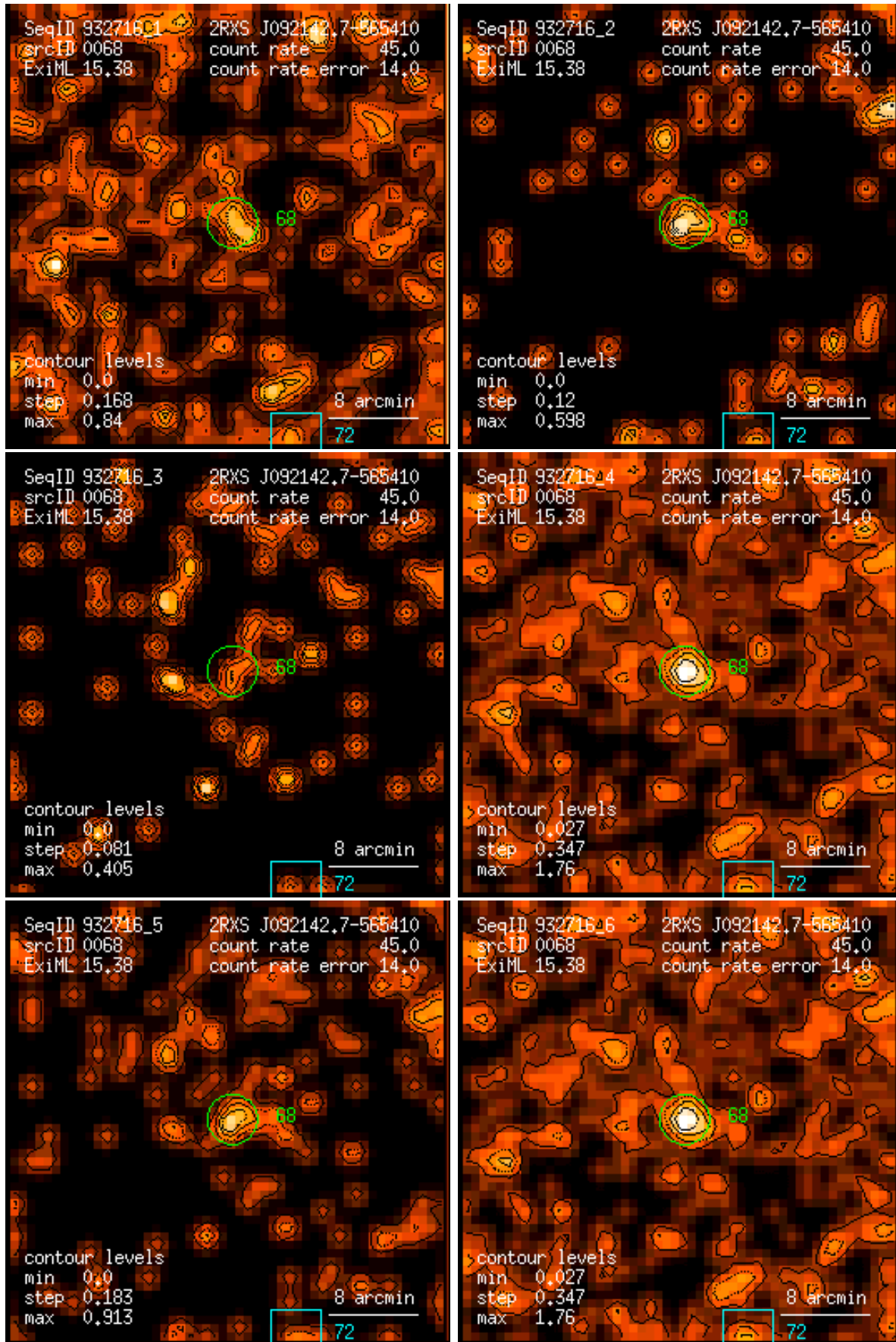
Figure 68: RASS 932716: detection 0068: band rate images, Gaussian filter: (1) PSPC channels 11 – 41, (2) 52 – 90, (3) 91 – 201, (4) 11 – 235, (5) 52 – 201, (6) 11 – 201. Broad band rates in counts/ks. Band rate contour levels in counts/ks/arcmin 2 .
