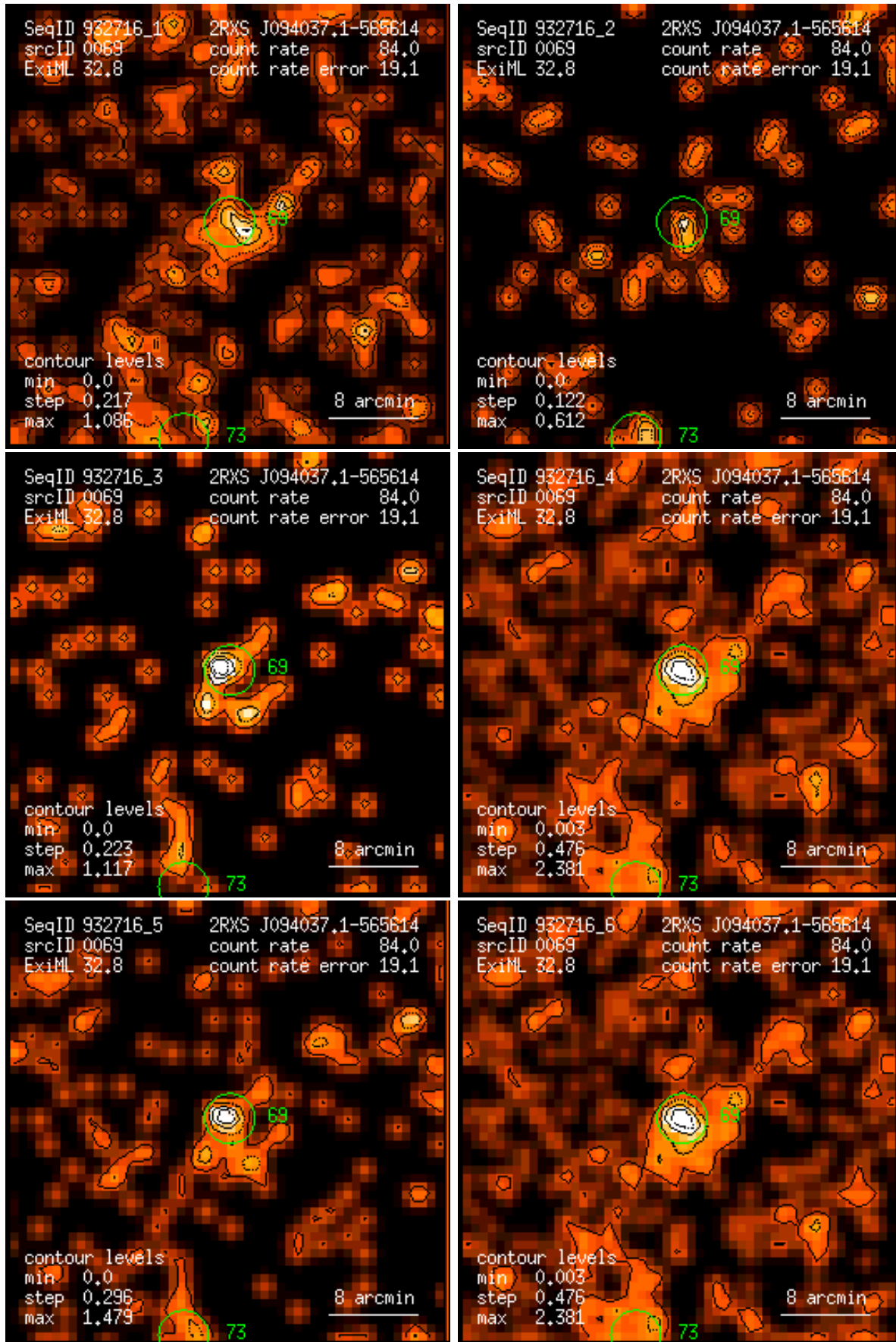
Figure 69: RASS 932716: detection 0069: band rate images, Gaussian filter: (1) PSPC channels 11 – 41, (2) 52 – 90, (3) 91 – 201, (4) 11 – 235, (5) 52 – 201, (6) 11 – 201. Broad band rates in counts/ks. Band rate contour levels in counts/ks/arcmin 2 .
