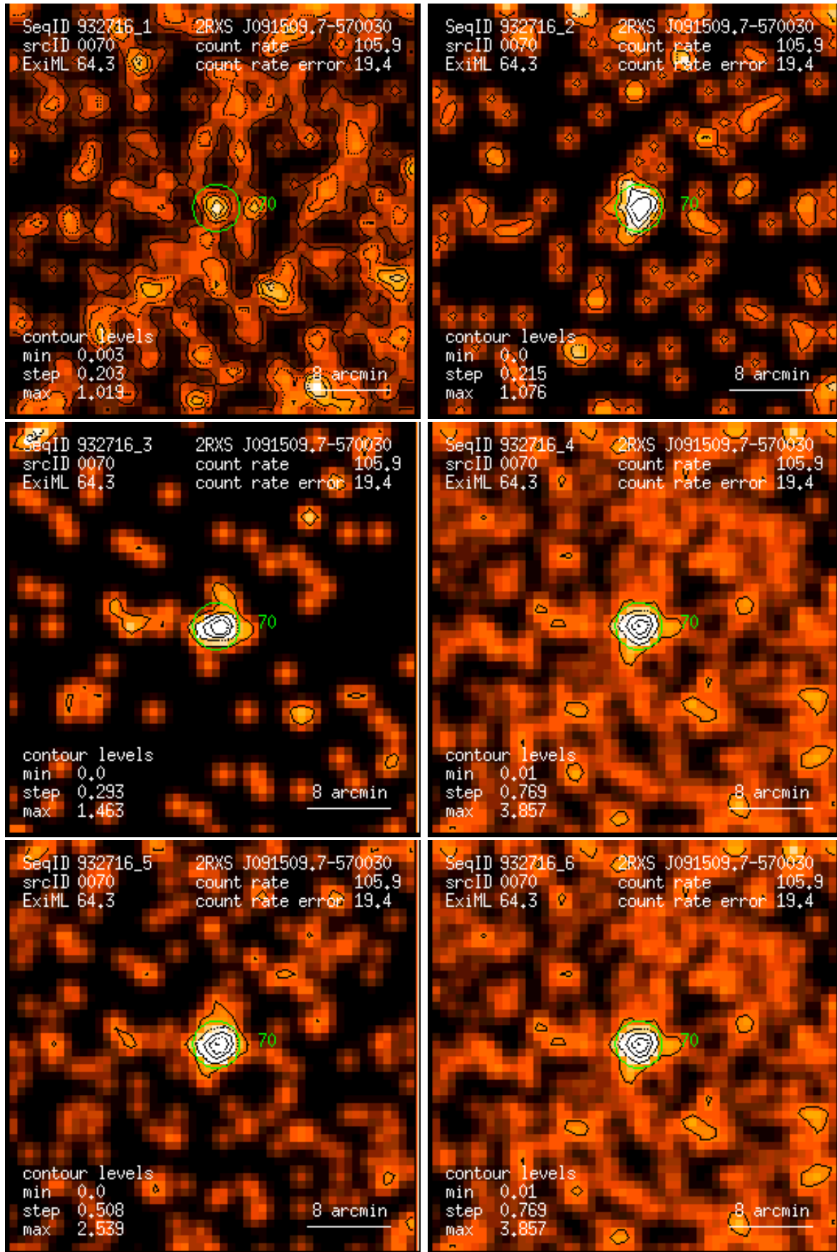
Figure 70: RASS 932716: detection 0070: band rate images, Gaussian filter: (1) PSPC channels 11 – 41, (2) 52 – 90, (3) 91 – 201, (4) 11 – 235, (5) 52 – 201, (6) 11 – 201. Broad band rates in counts/ks. Band rate contour levels in counts/ks/arcmin 2 .
