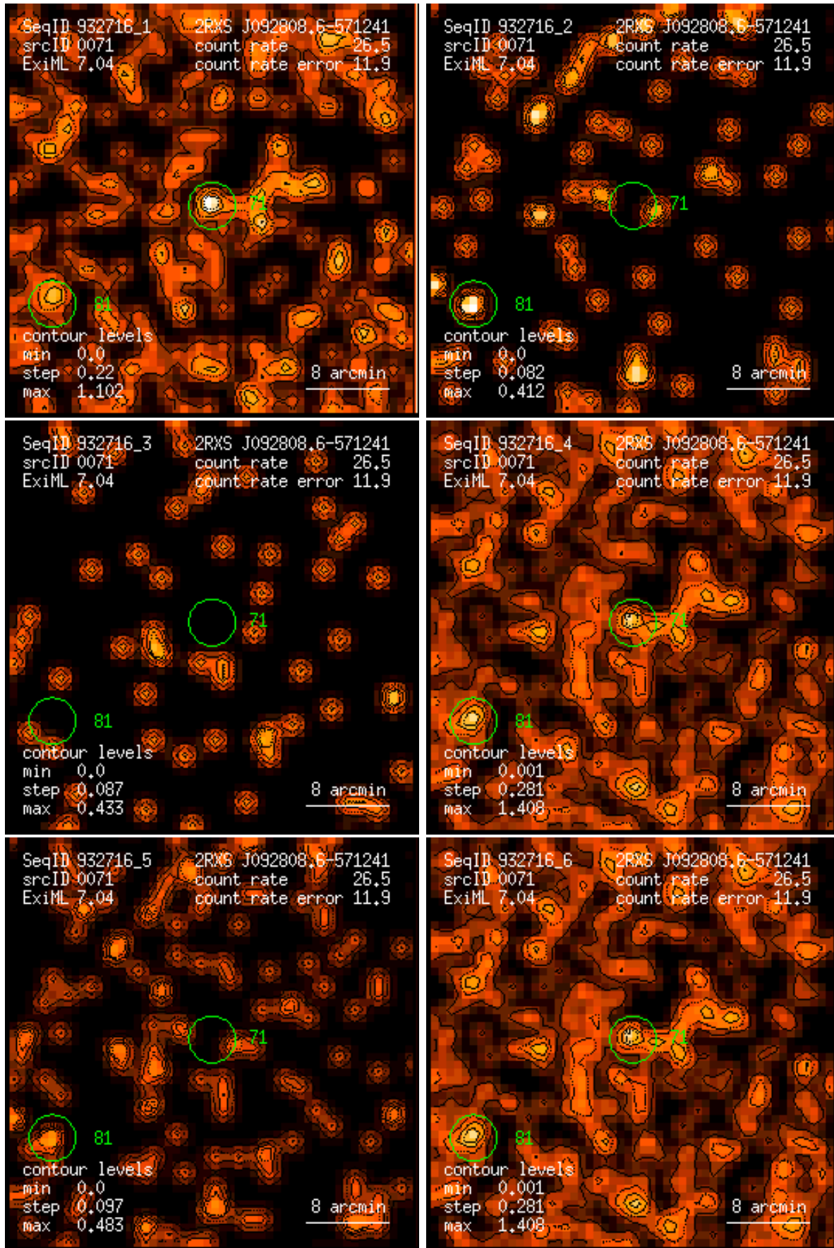
Figure 71: RASS 932716: detection 0071: band rate images, Gaussian filter: (1) PSPC channels 11 – 41, (2) 52 – 90, (3) 91 – 201, (4) 11 – 235, (5) 52 – 201, (6) 11 – 201. Broad band rates in counts/ks. Band rate contour levels in counts/ks/arcmin 2 .
