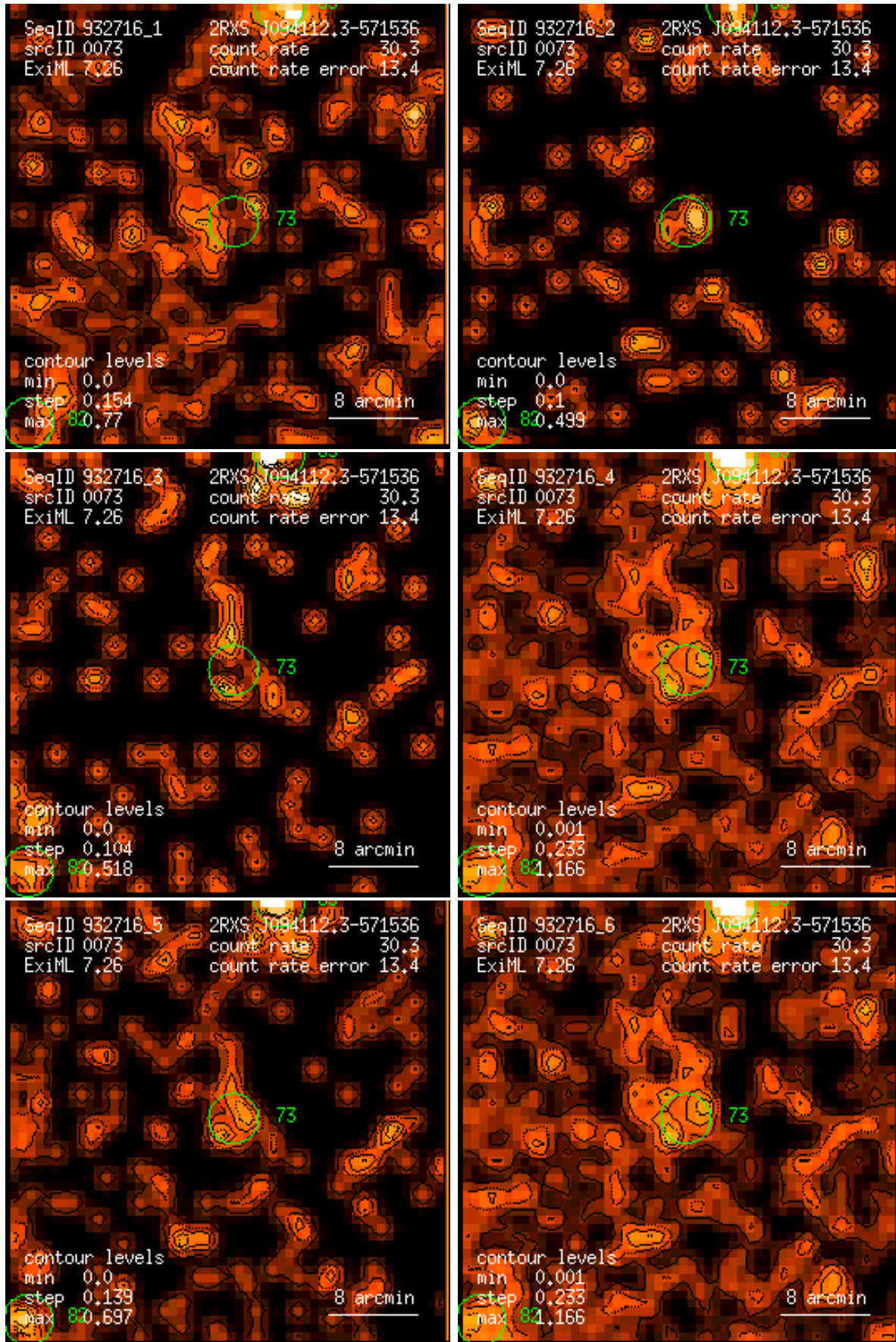
Figure 73: RASS 932716: detection 0073: band rate images, Gaussian filter: (1) PSPC channels 11 – 41, (2) 52 – 90, (3) 91 – 201, (4) 11 – 235, (5) 52 – 201, (6) 11 – 201. Broad band rates in counts/ks. Band rate contour levels in counts/ks/arcmin 2 .
