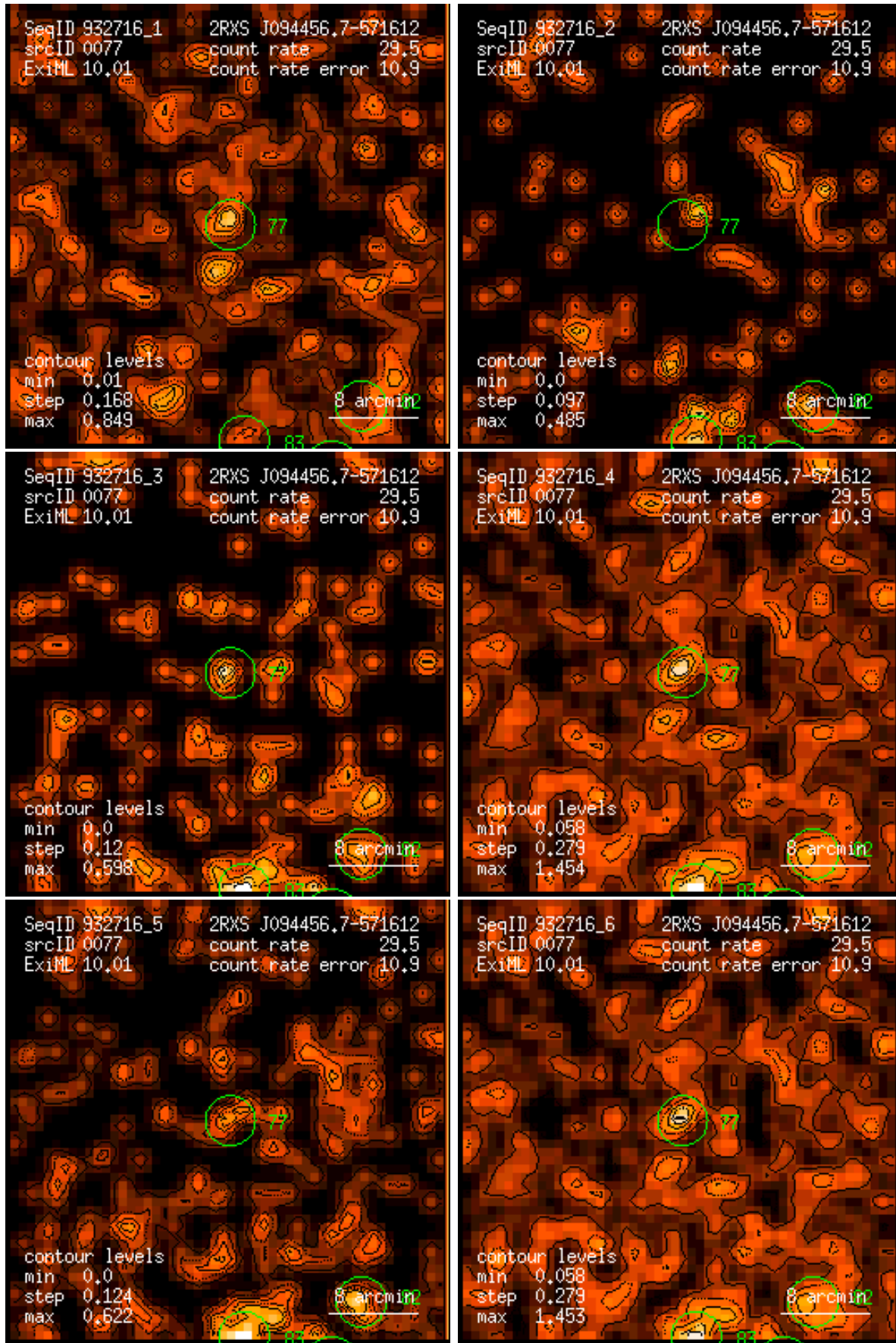
Figure 77: RASS 932716: detection 0077: band rate images, Gaussian filter: (1) PSPC channels 11 – 41, (2) 52 – 90, (3) 91 – 201, (4) 11 – 235, (5) 52 – 201, (6) 11 – 201. Broad band rates in counts/ks. Band rate contour levels in counts/ks/arcmin 2 .
