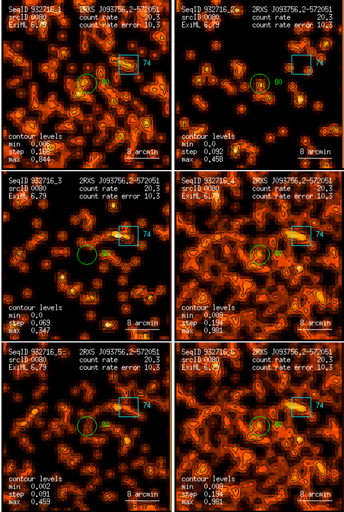
Figure 80: RASS 932716: detection 0080: band rate images, Gaussian filter: (1) PSPC channels 11 – 41, (2) 52 – 90, (3) 91 – 201, (4) 11 – 235, (5) 52 – 201, (6) 11 – 201. Broad band rates in counts/ks. Band rate contour levels in counts/ks/arcmin 2 .
