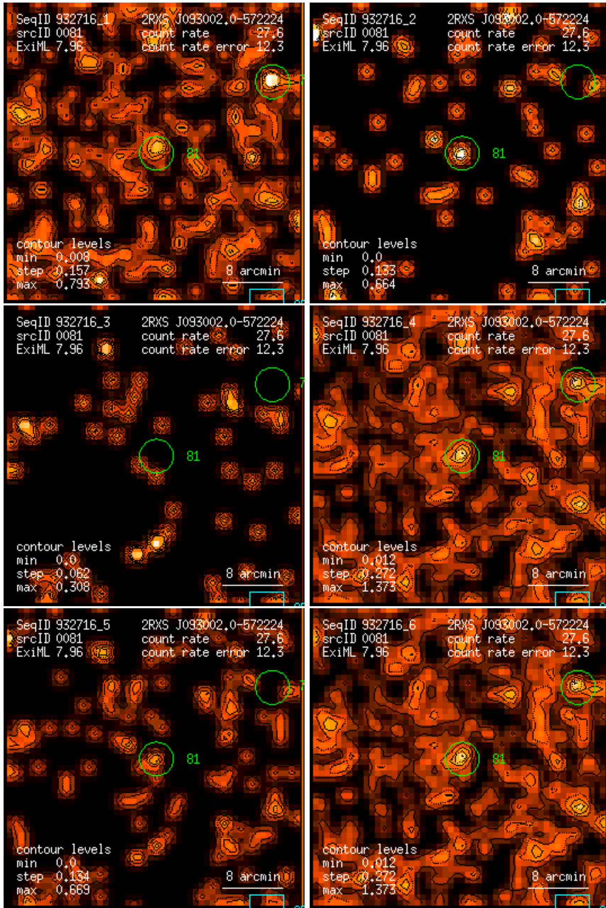
Figure 81: RASS 932716: detection 0081: band rate images, Gaussian filter: (1) PSPC channels 11 – 41, (2) 52 – 90, (3) 91 – 201, (4) 11 – 235, (5) 52 – 201, (6) 11 – 201. Broad band rates in counts/ks. Band rate contour levels in counts/ks/arcmin 2 .
