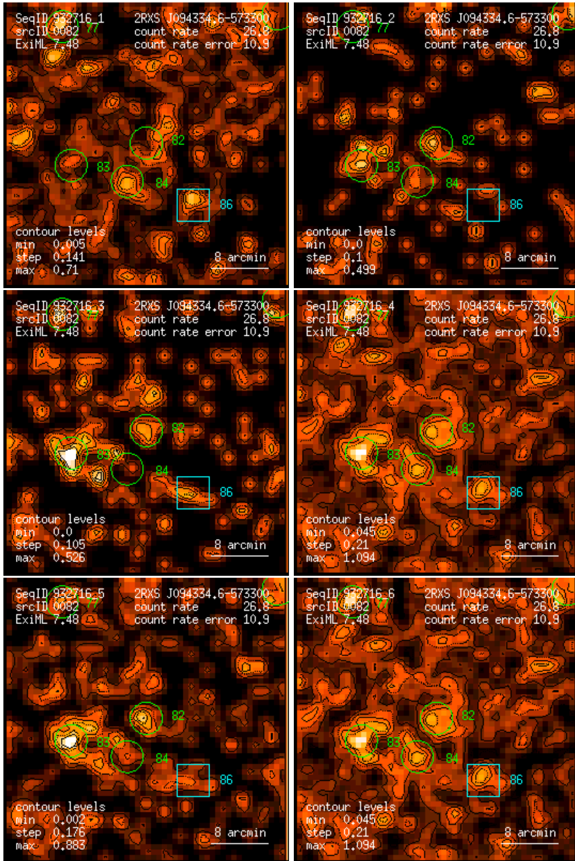
Figure 82: RASS 932716: detection 0082: band rate images, Gaussian filter: (1) PSPC channels 11 – 41, (2) 52 – 90, (3) 91 – 201, (4) 11 – 235, (5) 52 – 201, (6) 11 – 201. Broad band rates in counts/ks. Band rate contour levels in counts/ks/arcmin 2 .
