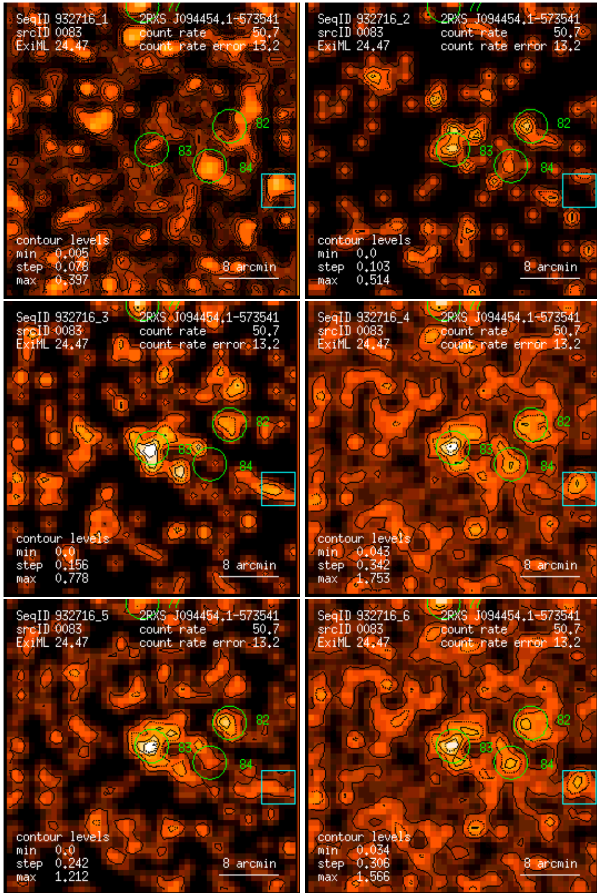
Figure 83: RASS 932716: detection 0083: band rate images, Gaussian filter: (1) PSPC channels 11 – 41, (2) 52 – 90, (3) 91 – 201, (4) 11 – 235, (5) 52 – 201, (6) 11 – 201. Broad band rates in counts/ks. Band rate contour levels in counts/ks/arcmin 2 .
