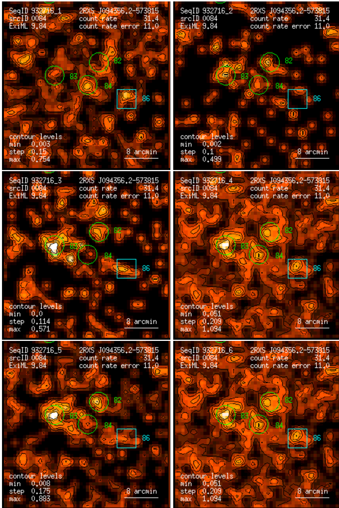
Figure 84: RASS 932716: detection 0084: band rate images, Gaussian filter: (1) PSPC channels 11 – 41, (2) 52 – 90, (3) 91 – 201, (4) 11 – 235, (5) 52 – 201, (6) 11 – 201. Broad band rates in counts/ks. Band rate contour levels in counts/ks/arcmin 2 .
